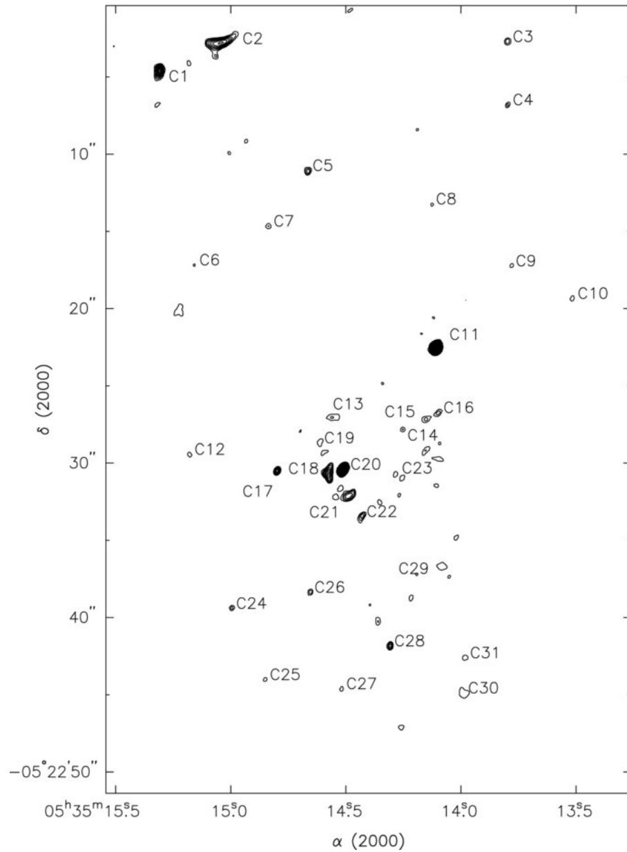
Figure 3. from A High Spatial Resolution Study of the \lambda = 3 mm Continuum of Orion-KL Friedel & Widicus Weaver 2011 ApJ 742 64 doi:10.1088/0004-637X/742/2/64 https://dx.doi.org/10.1088/0004-637X/742/2/64 © 2011. The American Astronomical Society. All rights reserved.
