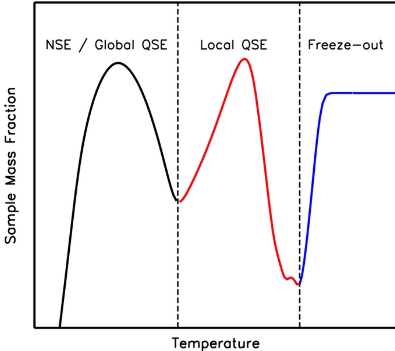
Figure 9. from Freeze-out Yields of Radioactivities in Core-collapse Supernovae Magkotsios, Timmes, & Wiescher 2011 ApJ 741 78 doi:10.1088/0004-637X/741/2/78 https://dx.doi.org/10.1088/0004-637X/741/2/78 © 2011. The American Astronomical Society. All rights reserved.
