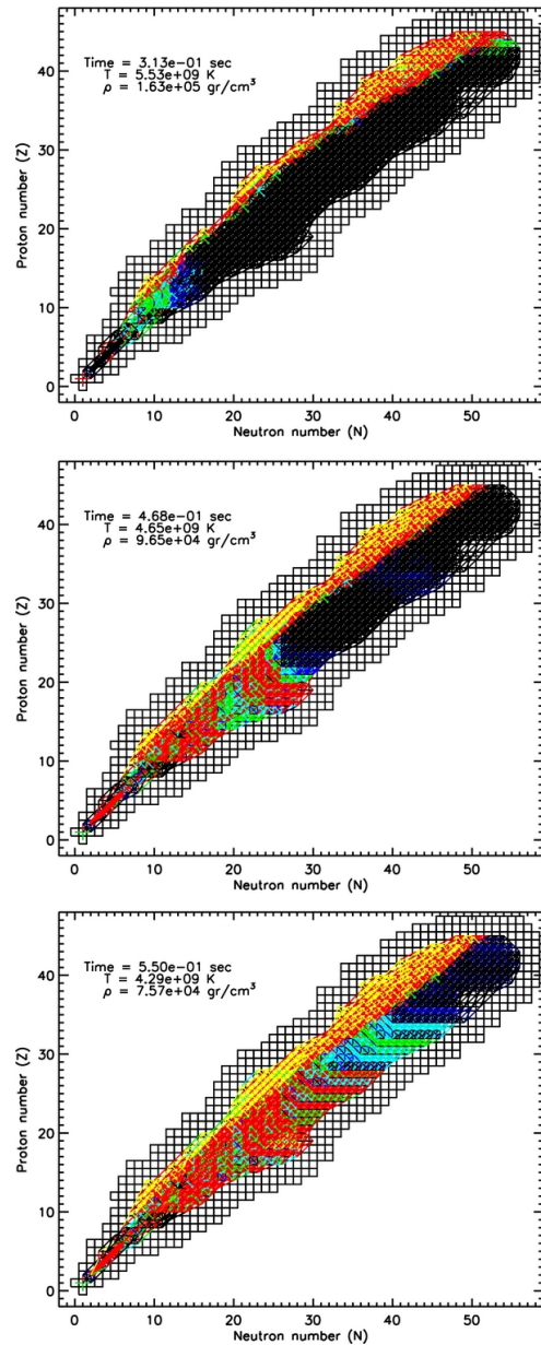
Figure 8. from Freeze-out Yields of Radioactivities in Core-collapse Supernovae Magkotsios, Timmes, & Wiescher 2011 ApJ 741 78 doi:10.1088/0004-637X/741/2/78 https://dx.doi.org/10.1088/0004-637X/741/2/78
