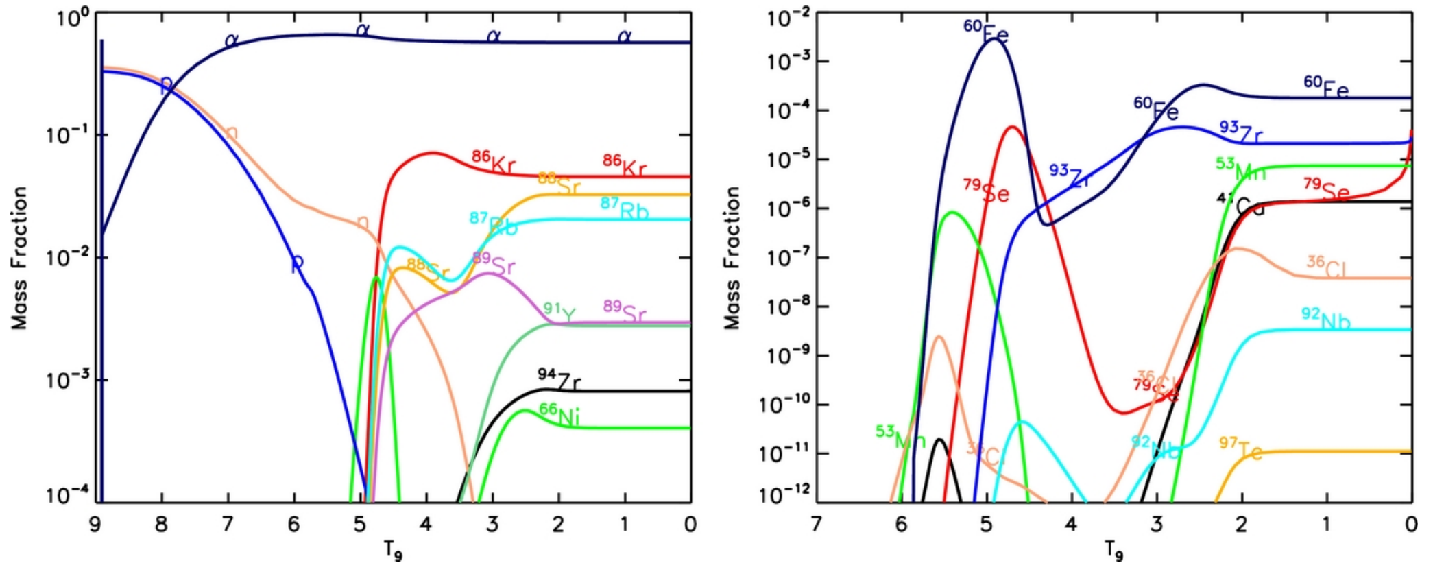
Figure 7. from Freeze-out Yields of Radioactivities in Core-collapse Supernovae Magkotsios, Timmes, & Wiescher 2011 ApJ 741 78 doi:10.1088/0004-637X/741/2/78 https://dx.doi.org/10.1088/0004-637X/741/2/78 © 2011. The American Astronomical Society. All rights reserved.
