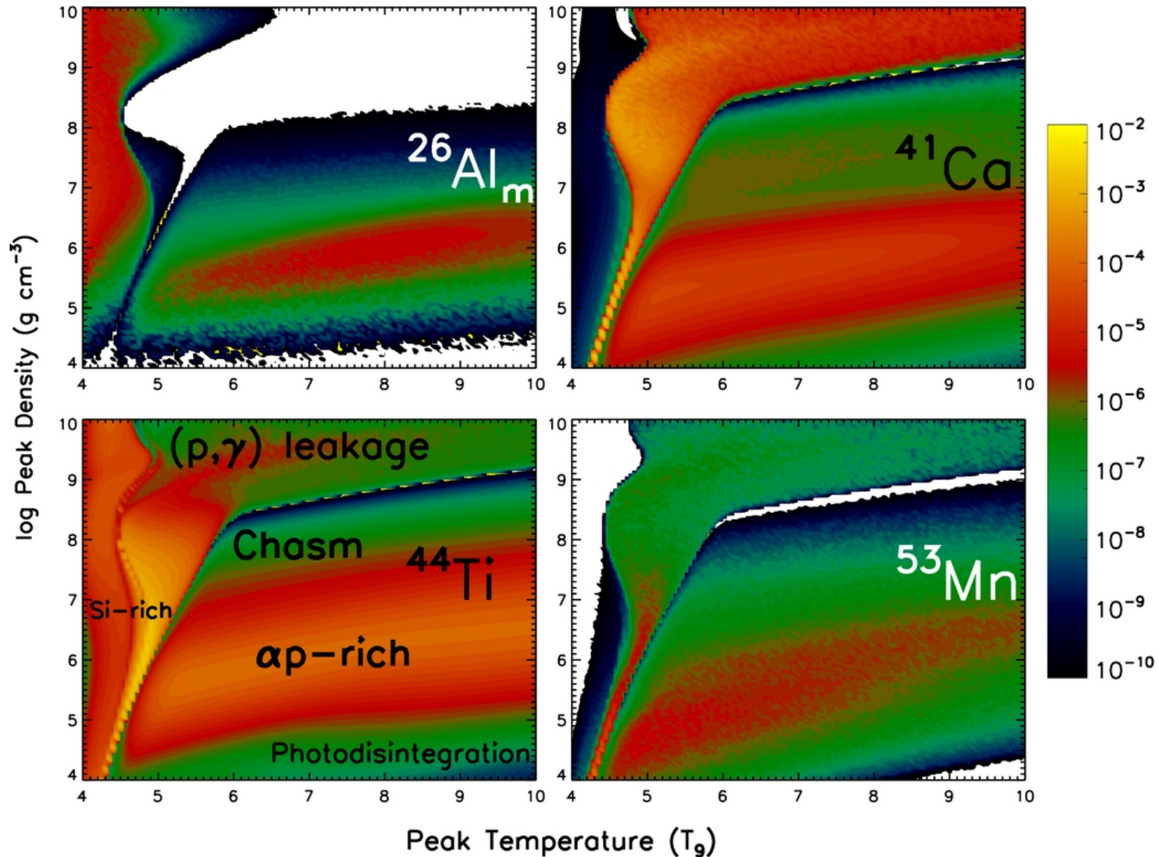
Figure 6. from Freeze-out Yields of Radioactivities in Core-collapse Supernovae Magkotsios, Timmes, & Wiescher 2011 ApJ 741 78 doi:10.1088/0004-637X/741/2/78 https://dx.doi.org/10.1088/0004-637X/741/2/78 © 2011. The American Astronomical Society. All rights reserved.
