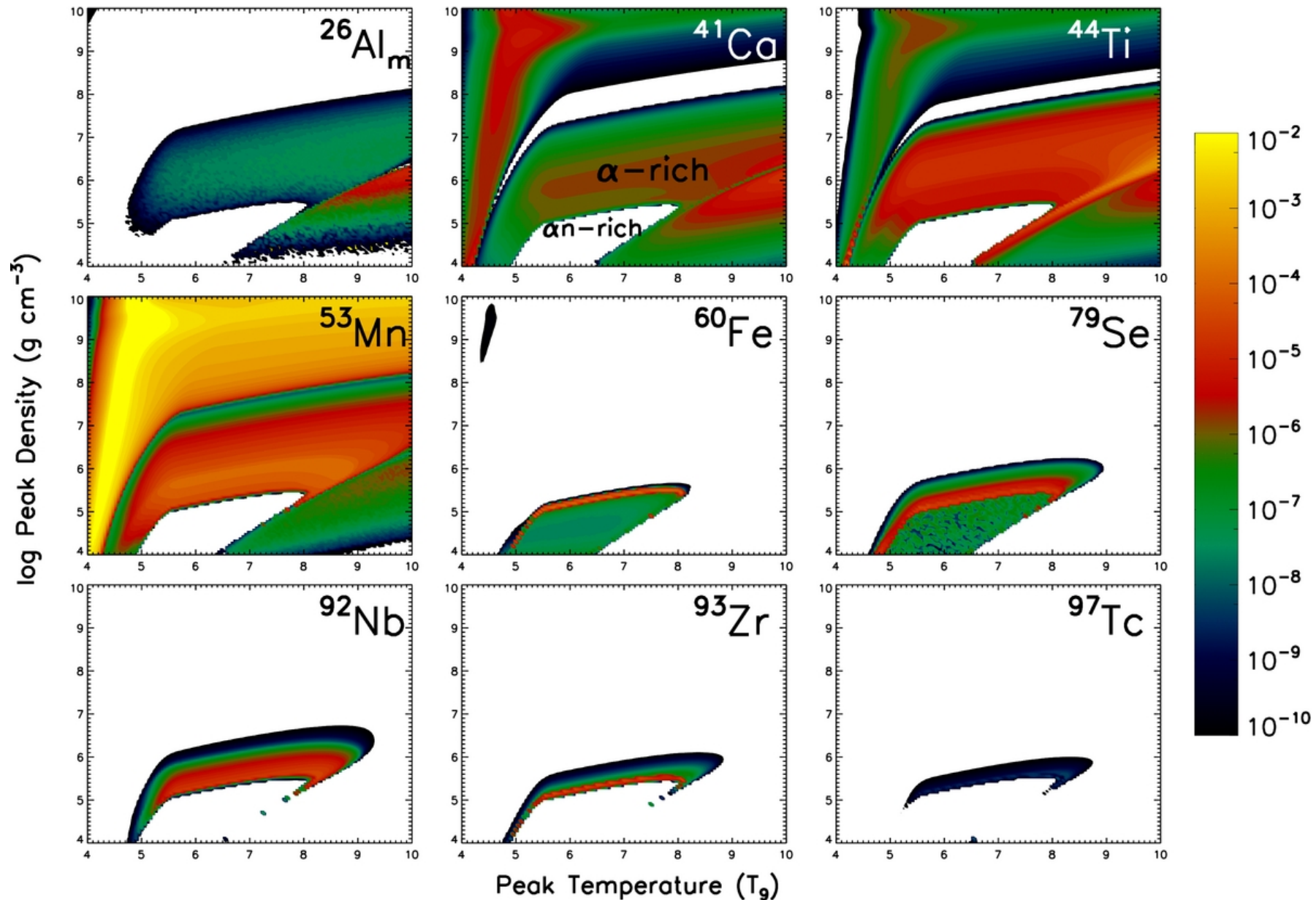
Figure 5. from Freeze-out Yields of Radioactivities in Core-collapse Supernovae Magkotsios, Timmes, & Wiescher 2011 ApJ 741 78 doi:10.1088/0004-637X/741/2/78 https://dx.doi.org/10.1088/0004-637X/741/2/78 © 2011. The American Astronomical Society. All rights reserved.
