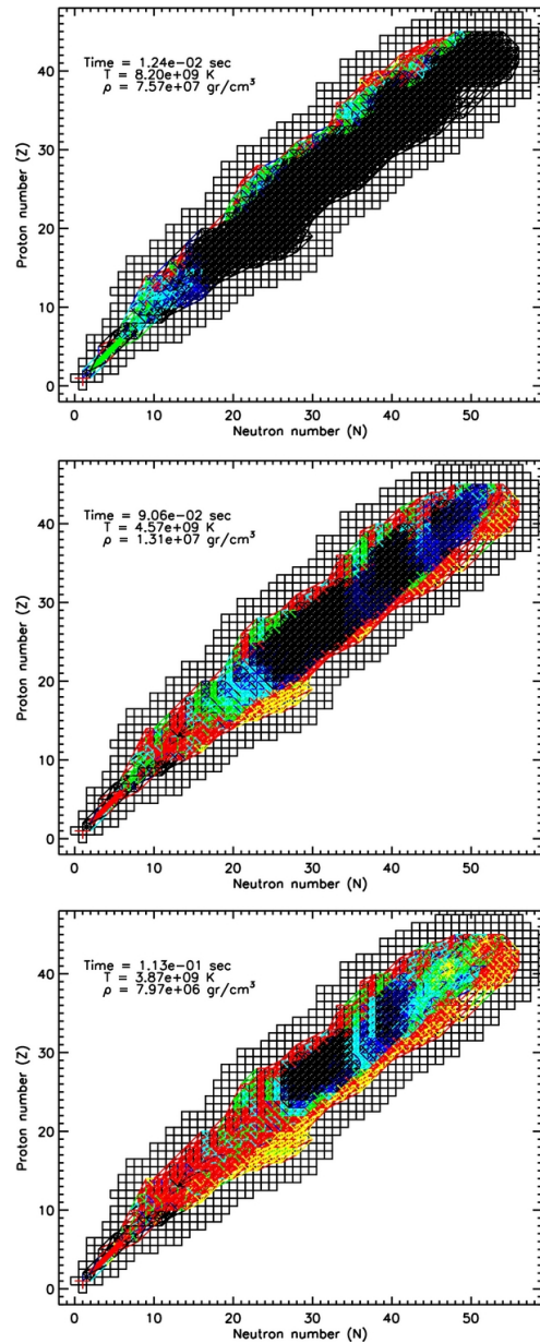
Figure 3. from Freeze-out Yields of Radioactivities in Core-collapse Supernovae Magkotsios, Timmes, & Wiescher 2011 ApJ 741 78 doi:10.1088/0004-637X/741/2/78 https://dx.doi.org/10.1088/0004-637X/741/2/78
