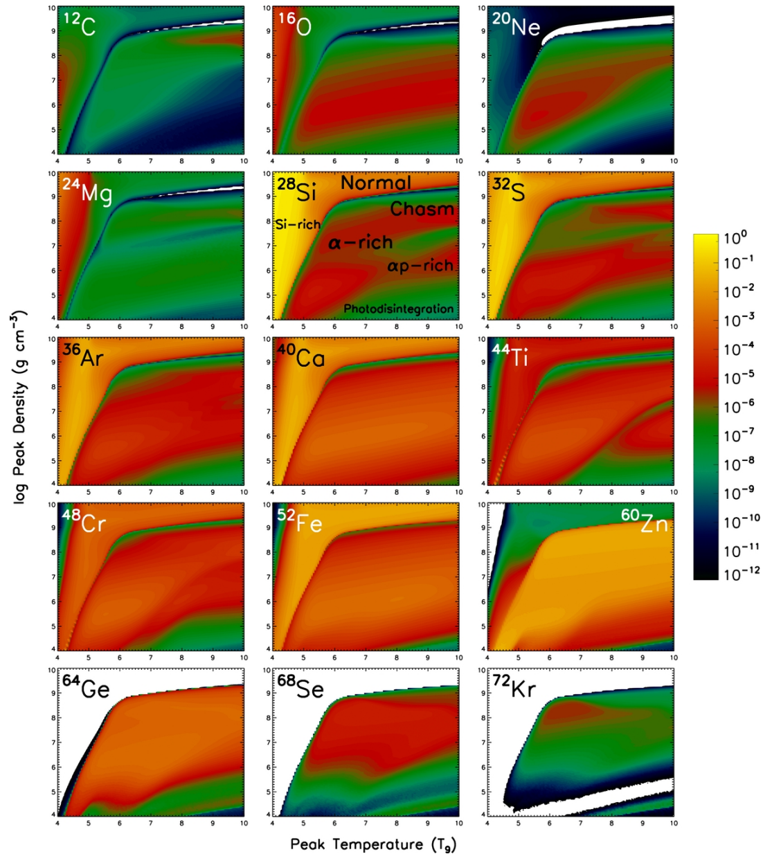
Figure 2. from Freeze-out Yields of Radioactivities in Core-collapse Supernovae Magkotsios, Timmes, & Wiescher 2011 ApJ 741 78 doi:10.1088/0004-637X/741/2/78 https://dx.doi.org/10.1088/0004-637X/741/2/78
