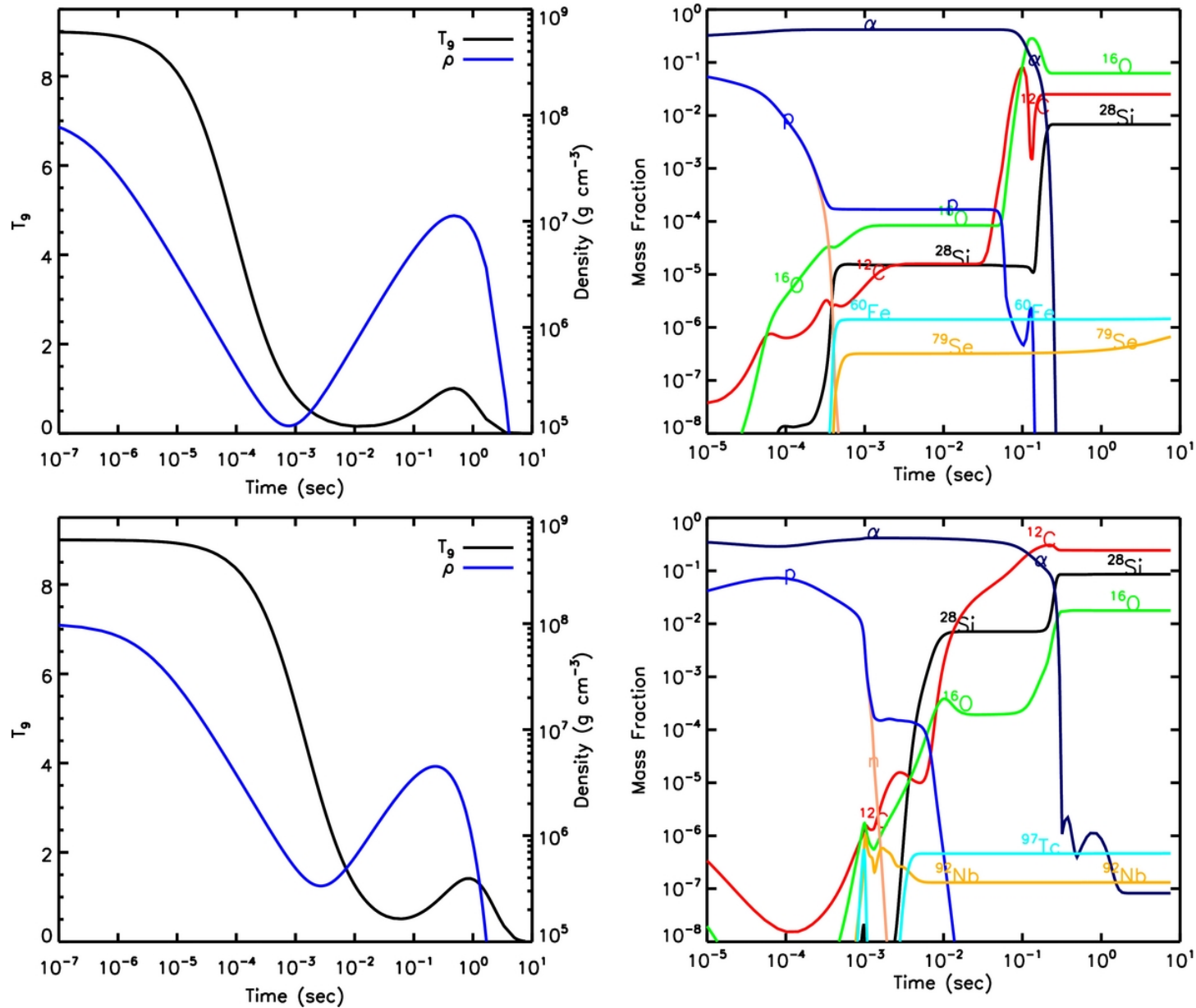
Figure 11. from Freeze-out Yields of Radioactivities in Core-collapse Supernovae Magkotsios, Timmes, & Wiescher 2011 ApJ 741 78 doi:10.1088/0004-637X/741/2/78 https://dx.doi.org/10.1088/0004-637X/741/2/78
