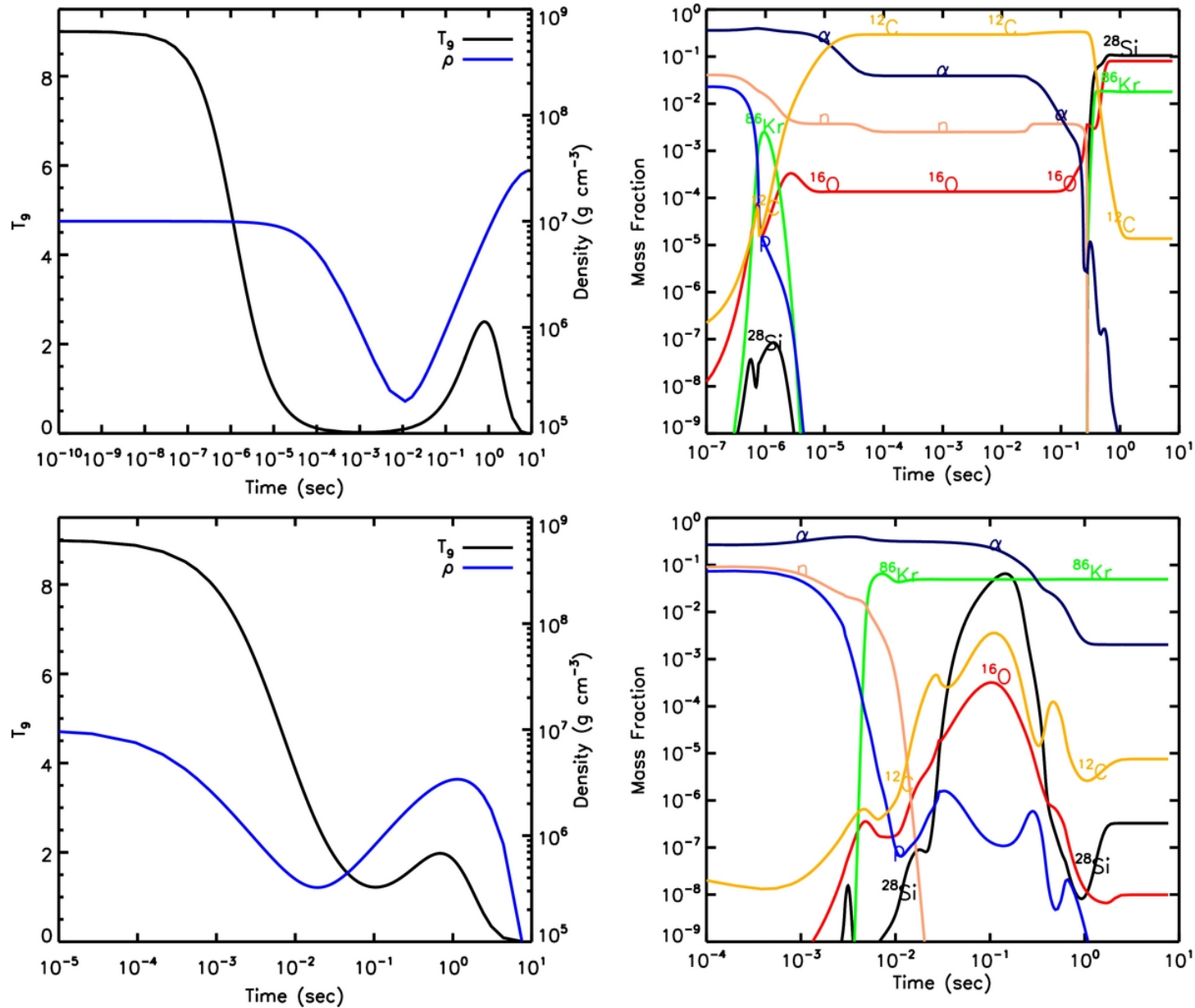
Figure 10. from Freeze-out Yields of Radioactivities in Core-collapse Supernovae Magkotsios, Timmes, & Wiescher 2011 ApJ 741 78 doi:10.1088/0004-637X/741/2/78 https://dx.doi.org/10.1088/0004-637X/741/2/78
