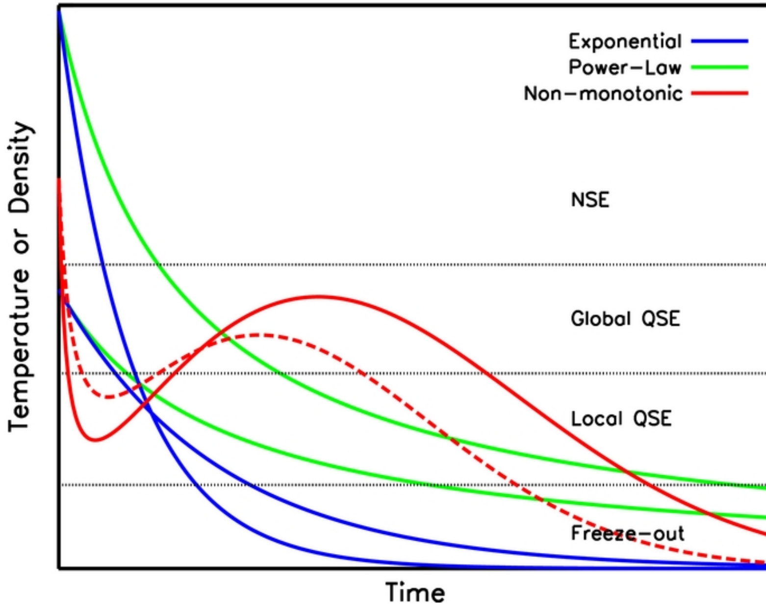
Figure 1. from Freeze-out Yields of Radioactivities in Core-collapse Supernovae Magkotsios, Timmes, & Wiescher 2011 ApJ 741 78 doi:10.1088/0004-637X/741/2/78 https://dx.doi.org/10.1088/0004-637X/741/2/78 © 2011. The American Astronomical Society. All rights reserved.
