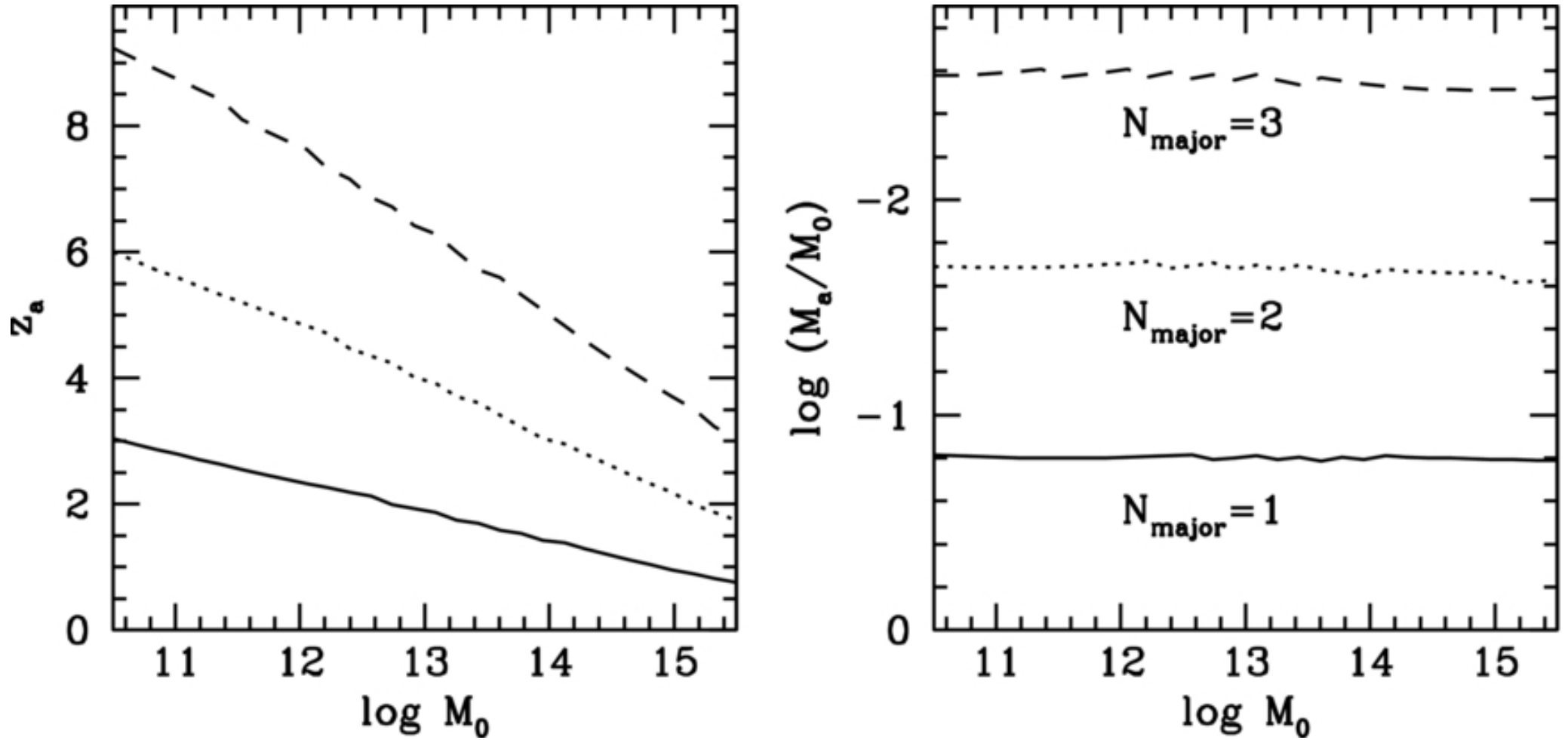
Figure 6. from An Analytical Model for the Accretion of Dark Matter Subhalos Yang et al. 2011 ApJ 741 13 doi:10.1088/0004-637X/741/1/13 https://dx.doi.org/10.1088/0004-637X/741/1/13 © 2011. The American Astronomical Society. All rights reserved.
