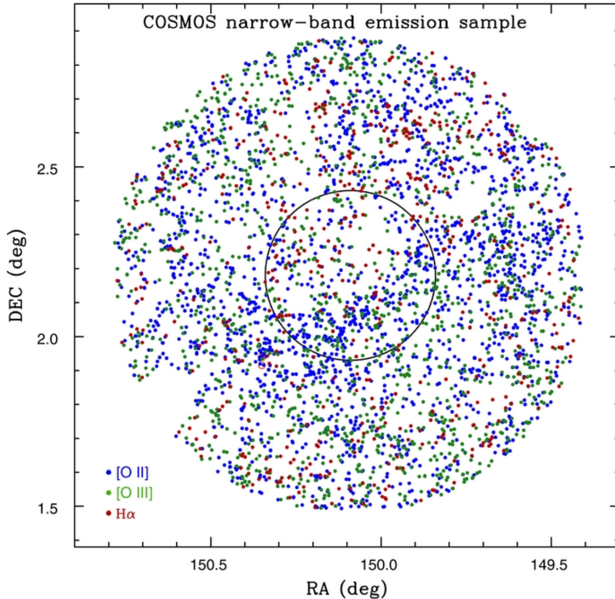
Figure 5. from Detections of Faint Ly Emitters at z = 5.7 : Galaxy Building Blocks and Engines of Reionization Dressler et al. 2011 ApJ 740 71 doi:10.1088/0004-637X/740/2/71 https://dx.doi.org/10.1088/0004-637X/740/2/71 © 2011. The American Astronomical Society. All rights reserved.
