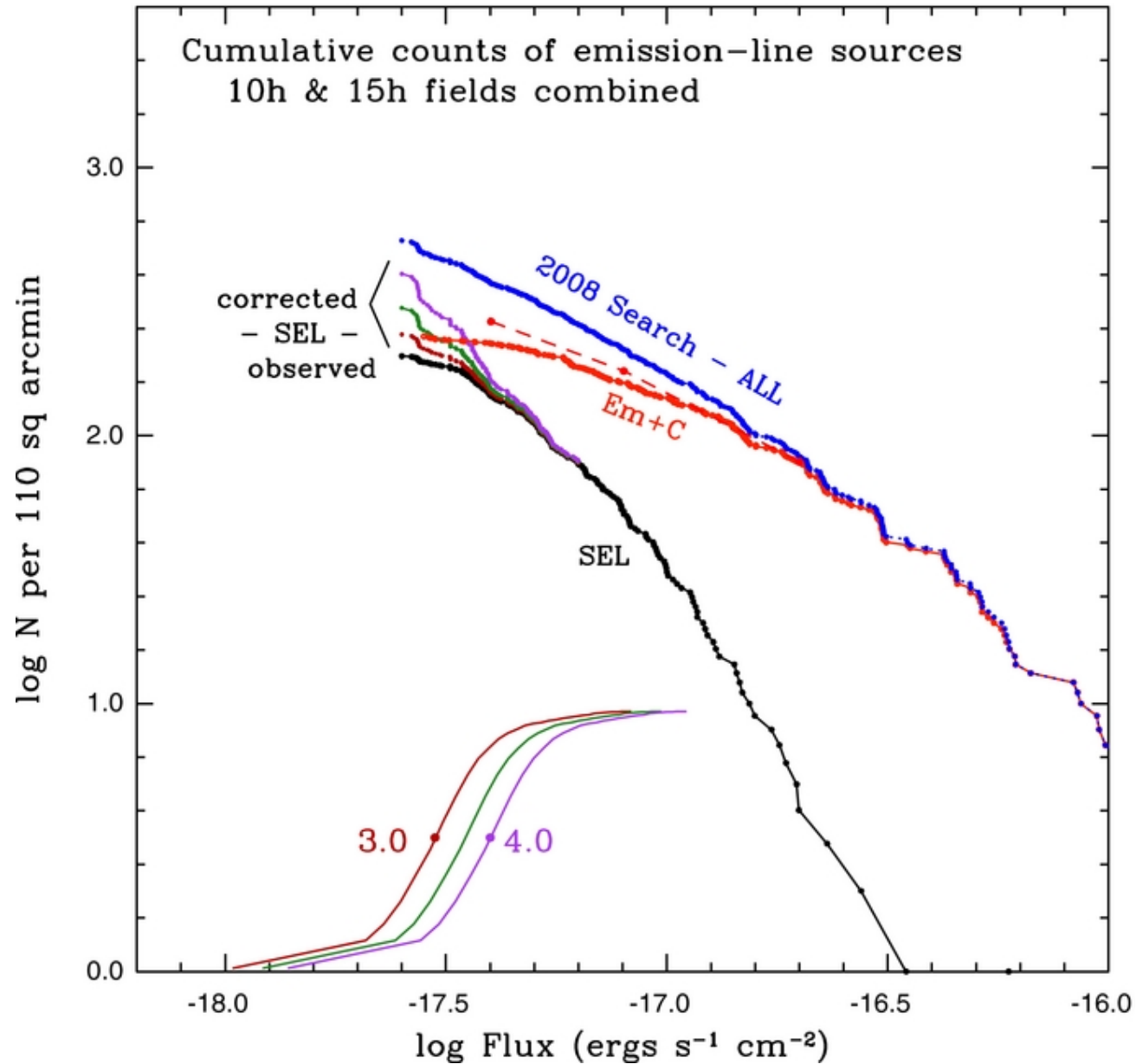
Figure 4. from Detections of Faint Ly Emitters at z = 5.7 : Galaxy Building Blocks and Engines of Reionization Dressler et al. 2011 ApJ 740 71 doi:10.1088/0004-637X/740/2/71 https://dx.doi.org/10.1088/0004-637X/740/2/71 © 2011. The American Astronomical Society. All rights reserved.
