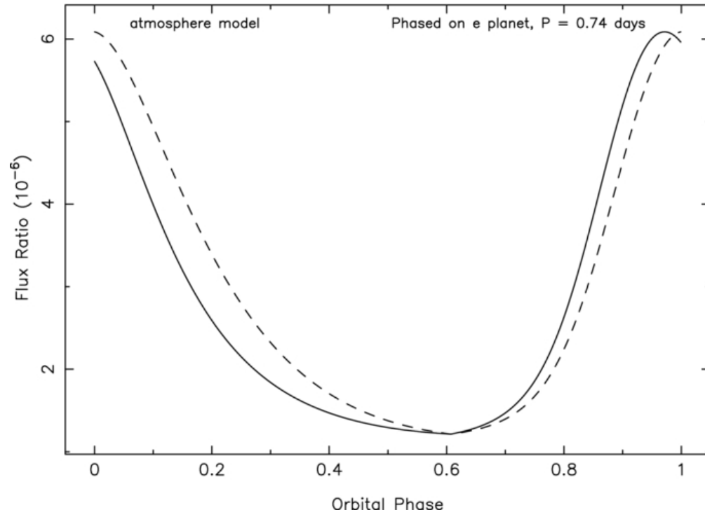
Figure 3. from Planetary Phase Variations of the 55 Cancri System Kane et al. 2011 ApJ 740 61 doi:10.1088/0004-637X/740/2/61 https://dx.doi.org/10.1088/0004-637X/740/2/61 © 2011. The American Astronomical Society. All rights reserved.
