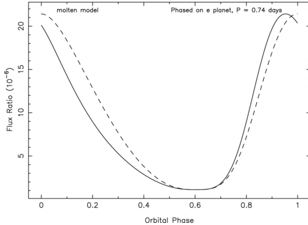
Figure 2. from Planetary Phase Variations of the 55 Cancri System Kane et al. 2011 ApJ 740 61 doi:10.1088/0004-637X/740/2/61 https://dx.doi.org/10.1088/0004-637X/740/2/61 © 2011. The American Astronomical Society. All rights reserved.
