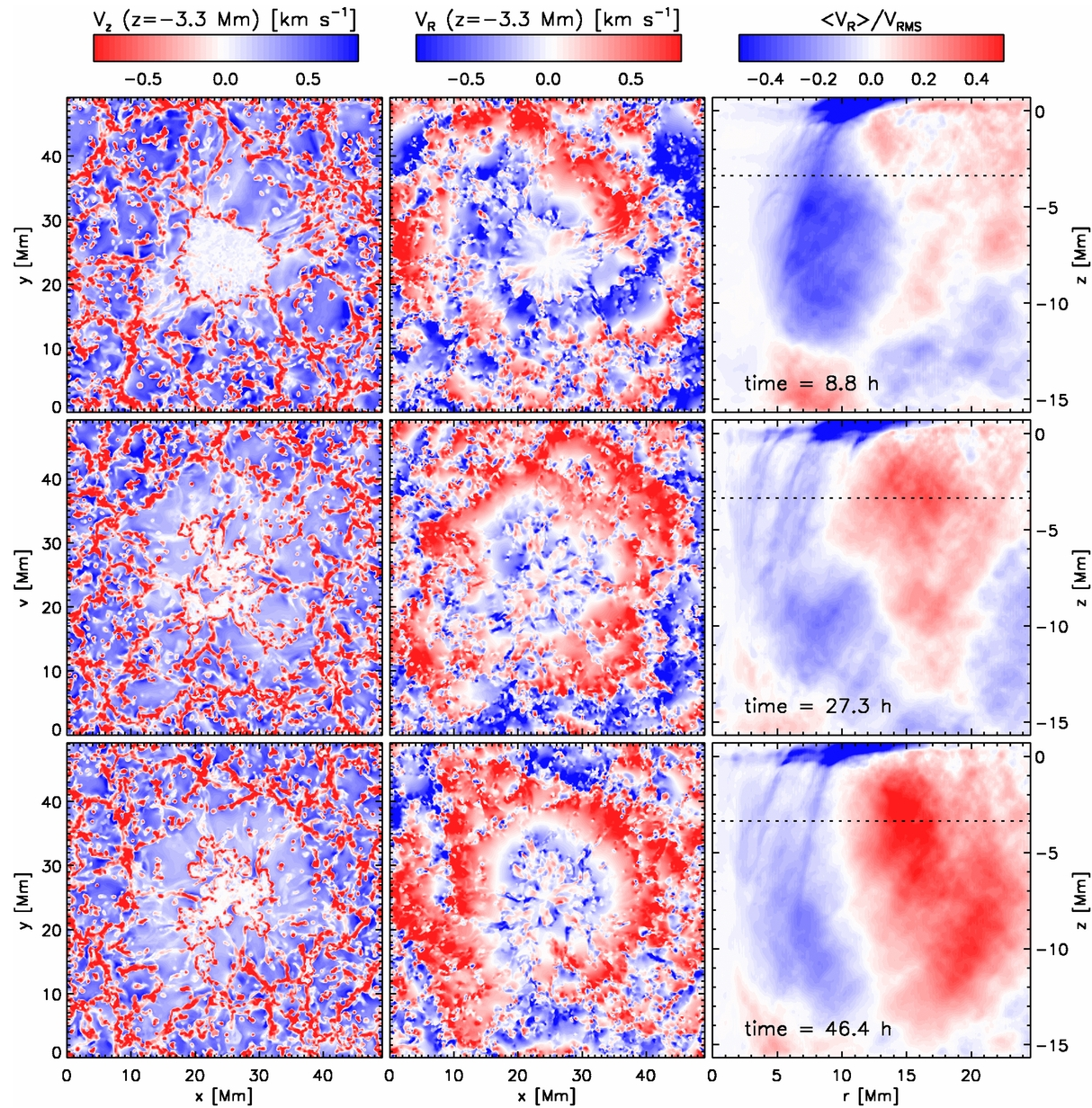
Figure 2. from Subsurface Magnetic Field and Flow Structure of Simulated Sunspots Rempel 2011 ApJ 740 15 doi:10.1088/0004-637X/740/1/15 https://dx.doi.org/10.1088/0004-637X/740/1/15
