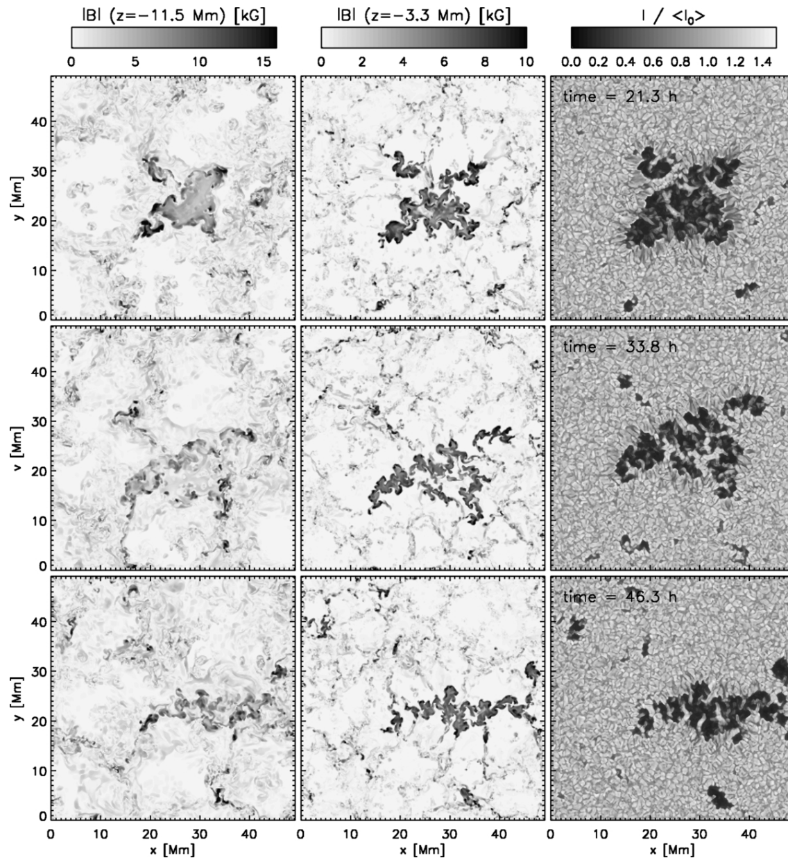
Figure 13. from Subsurface Magnetic Field and Flow Structure of Simulated Sunspots Rempel 2011 ApJ 740 15 doi:10.1088/0004-637X/740/1/15 https://dx.doi.org/10.1088/0004-637X/740/1/15
