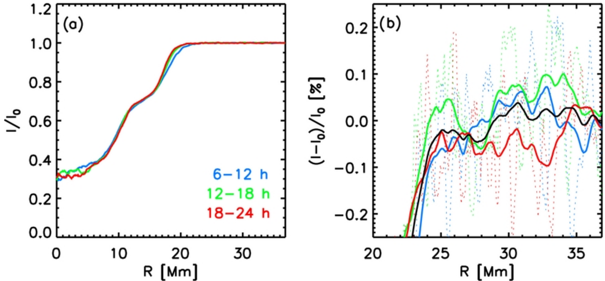
Figure 11. from Subsurface Magnetic Field and Flow Structure of Simulated Sunspots Rempel 2011 ApJ 740 15 doi:10.1088/0004-637X/740/1/15 https://dx.doi.org/10.1088/0004-637X/740/1/15 © 2011. The American Astronomical Society. All rights reserved.
