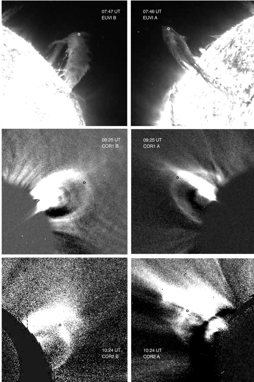
Figure 6. from Acceleration of Coronal Mass Ejections from Three-dimensional Reconstruction of STEREO Images Joshi & Srivastava 2011 ApJ 739 8 doi:10.1088/0004-637X/739/1/8 https://dx.doi.org/10.1088/0004-637X/739/1/8 © 2011. The American Astronomical Society. All rights reserved.
