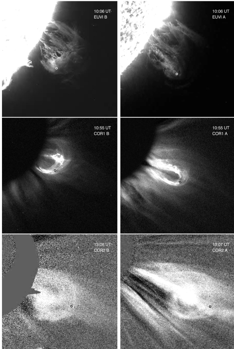
Figure 3. from Acceleration of Coronal Mass Ejections from Three-dimensional Reconstruction of STEREO Images Joshi & Srivastava 2011 ApJ 739 8 doi:10.1088/0004-637X/739/1/8 https://dx.doi.org/10.1088/0004-637X/739/1/8 © 2011. The American Astronomical Society. All rights reserved.
