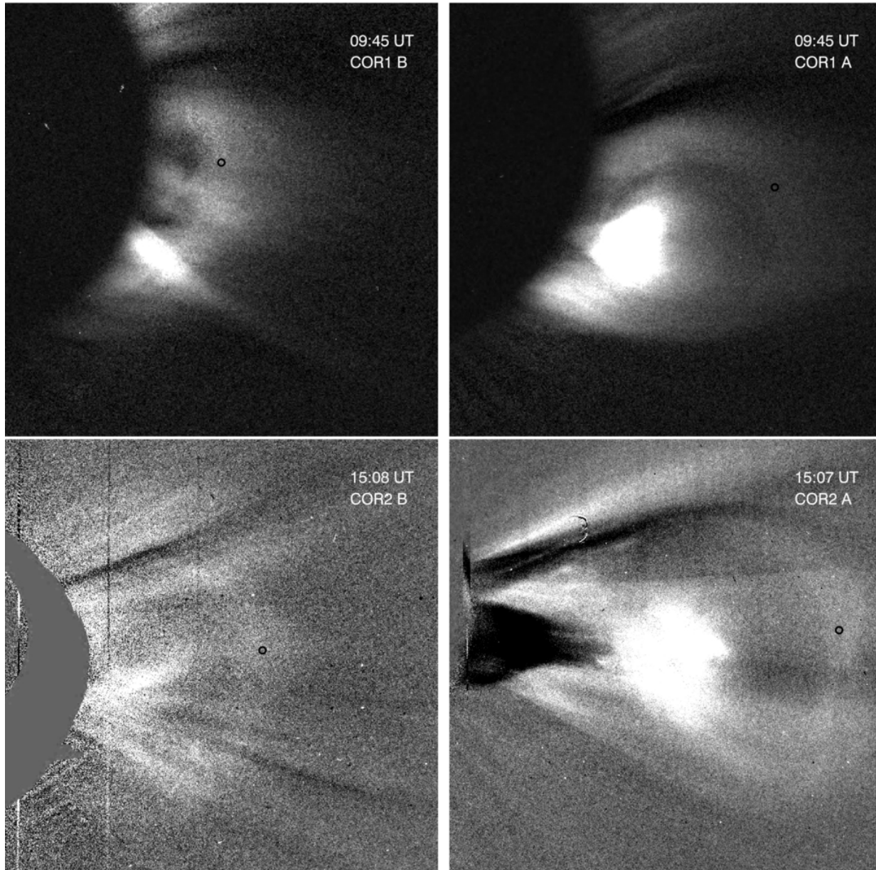
Figure 1. from Acceleration of Coronal Mass Ejections from Three-dimensional Reconstruction of STEREO Images Joshi & Srivastava 2011 ApJ 739 8 doi:10.1088/0004-637X/739/1/8 https://dx.doi.org/10.1088/0004-637X/739/1/8 © 2011. The American Astronomical Society. All rights reserved.
