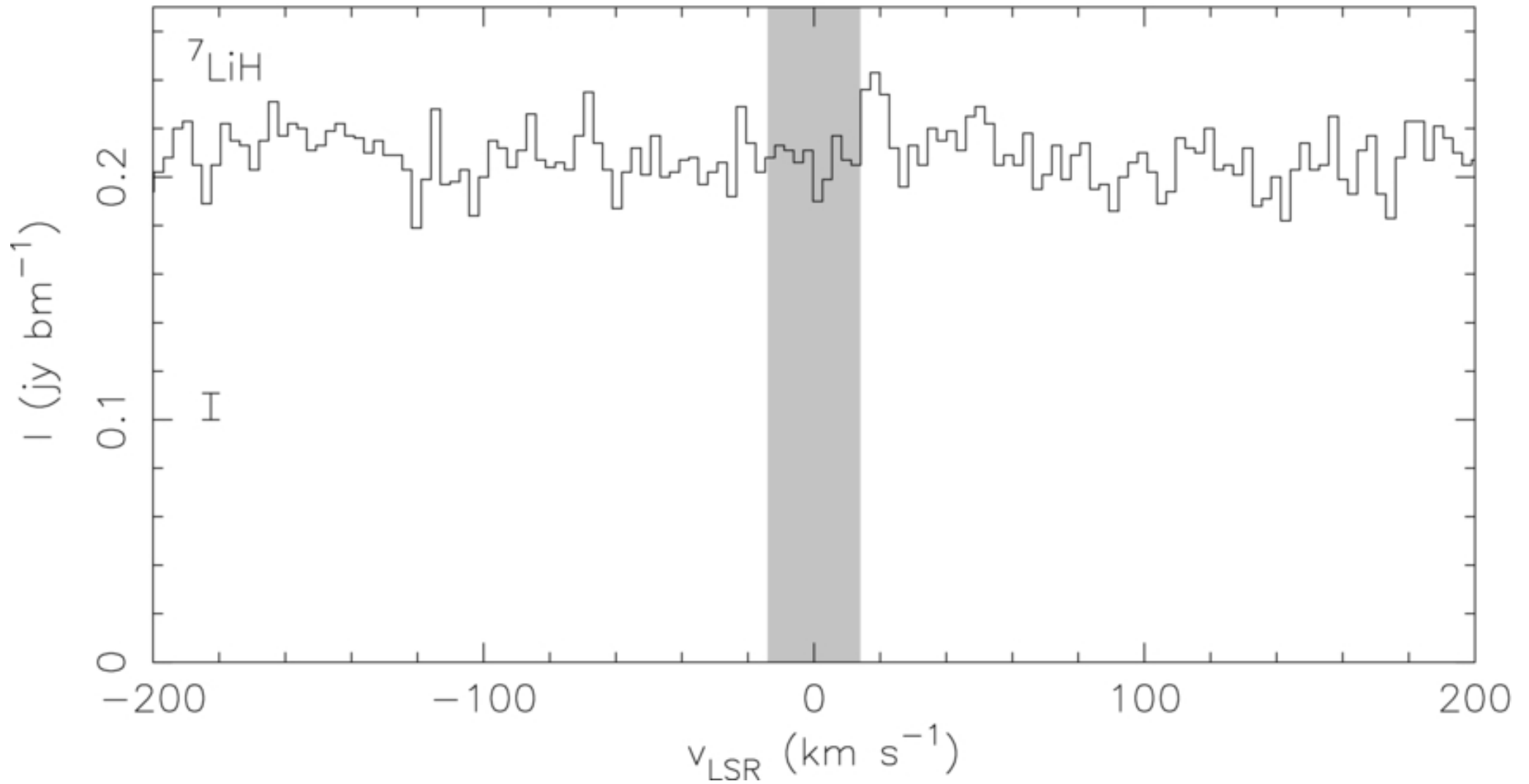
Figure 8. from The Search for Extragalactic Lithium Hydride Friedel, Kemball, & Fields 2011 ApJ 738 37 doi:10.1088/0004-637X/738/1/37 https://dx.doi.org/10.1088/0004-637X/738/1/37 © 2011. The American Astronomical Society. All rights reserved.
