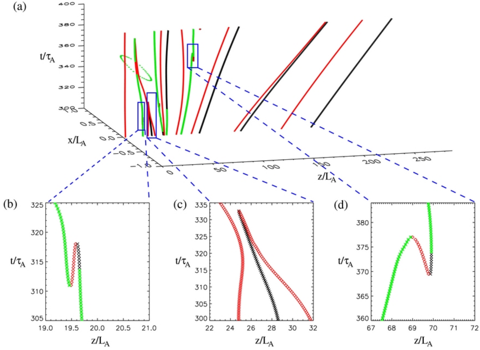
Figure 8. from Spontaneous Current-layer Fragmentation and Cascading Reconnection in Solar Flares. I. Model and Analysis Bárta et al. 2011 ApJ 737 24 doi:10.1088/0004-637X/737/1/24 https://dx.doi.org/10.1088/0004-637X/737/1/24 © 2011. The American Astronomical Society. All rights reserved.
