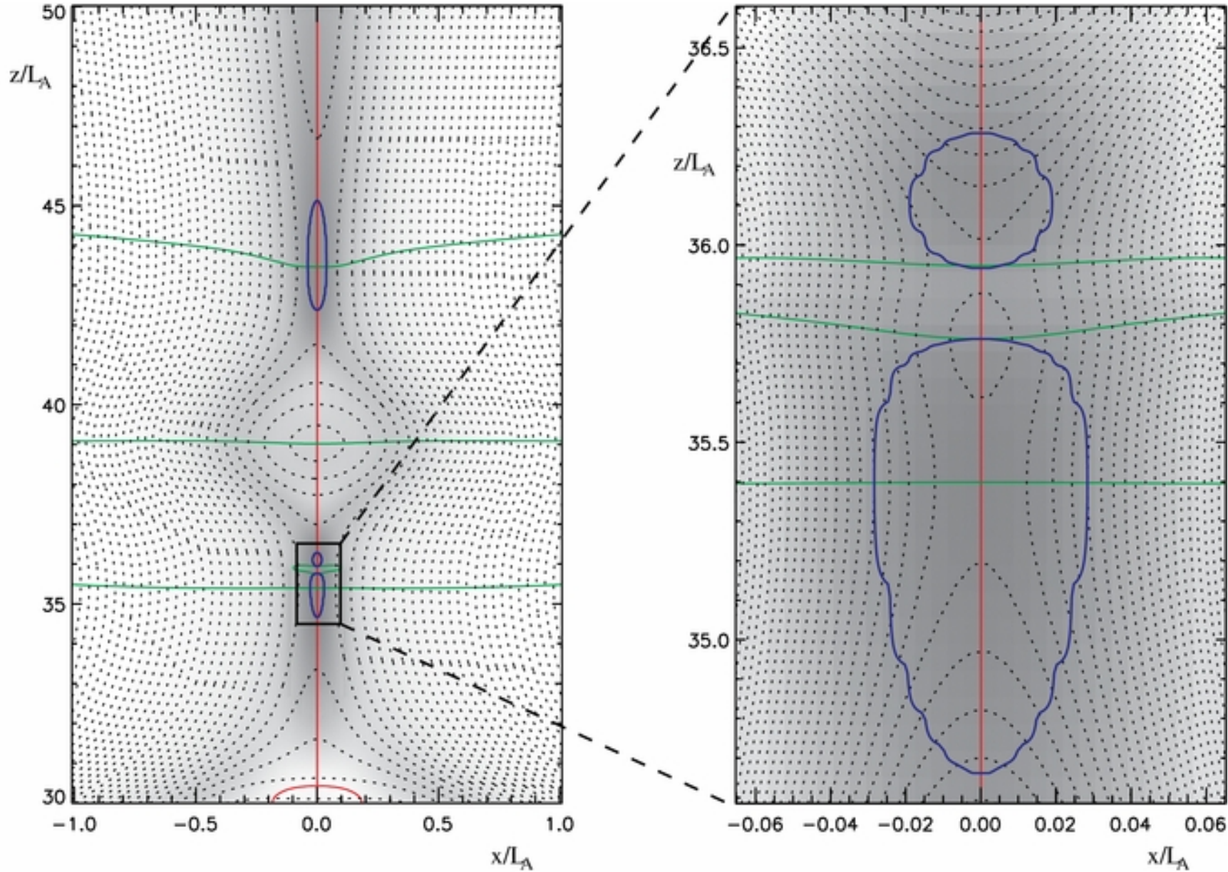
Figure 7. from Spontaneous Current-layer Fragmentation and Cascading Reconnection in Solar Flares. I. Model and Analysis Bárta et al. 2011 ApJ 737 24 doi:10.1088/0004-637X/737/1/24 https://dx.doi.org/10.1088/0004-637X/737/1/24 © 2011. The American Astronomical Society. All rights reserved.
