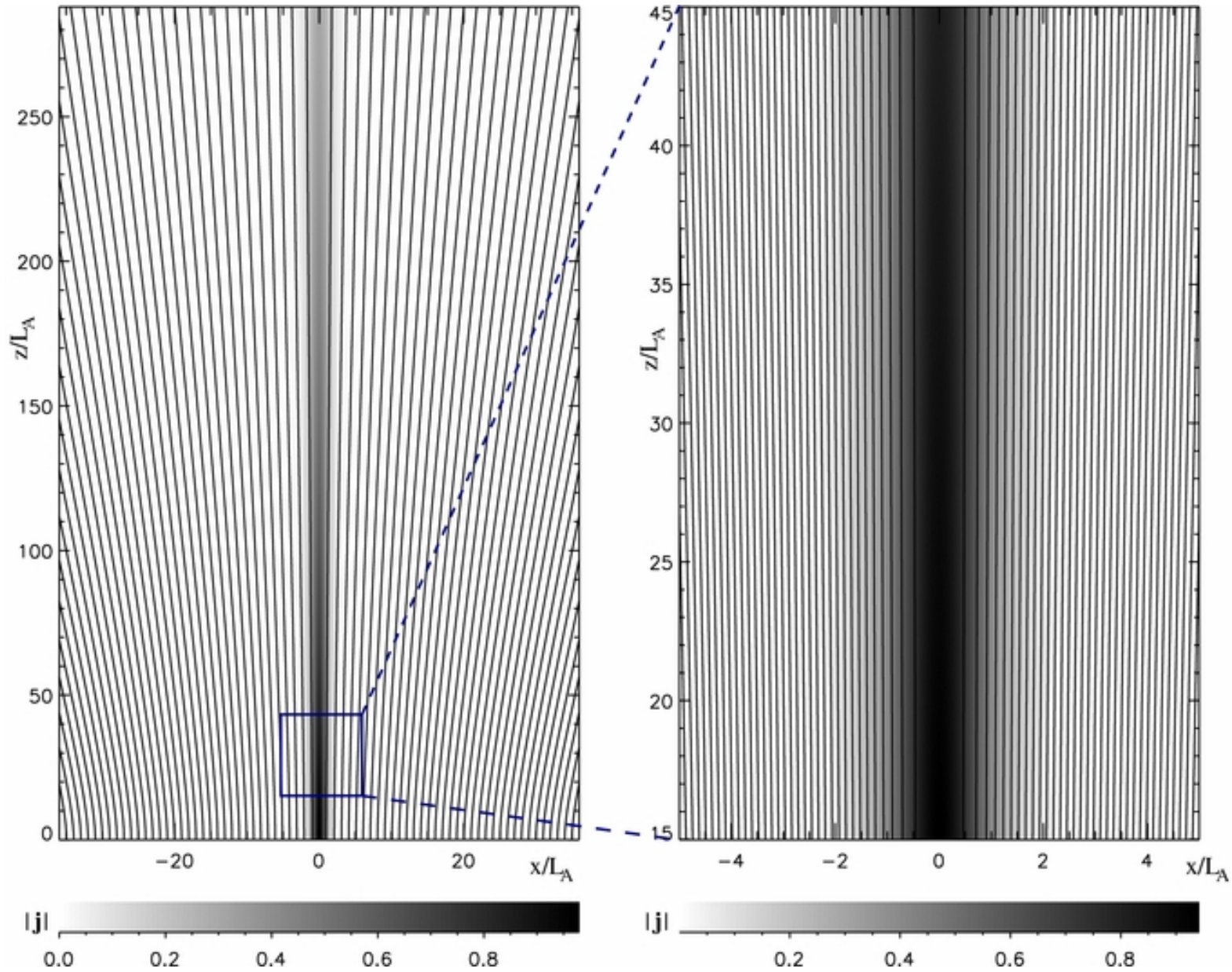
Figure 3. from Spontaneous Current-layer Fragmentation and Cascading Reconnection in Solar Flares. I. Model and Analysis Bárta et al. 2011 ApJ 737 24 doi:10.1088/0004-637X/737/1/24 https://dx.doi.org/10.1088/0004-637X/737/1/24 © 2011. The American Astronomical Society. All rights reserved.
