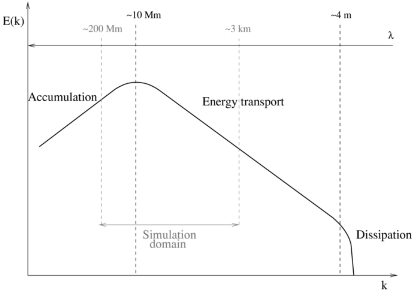
Figure 1. from Spontaneous Current-layer Fragmentation and Cascading Reconnection in Solar Flares. I. Model and Analysis Bárta et al. 2011 ApJ 737 24 doi:10.1088/0004-637X/737/1/24 https://dx.doi.org/10.1088/0004-637X/737/1/24 © 2011. The American Astronomical Society. All rights reserved.
