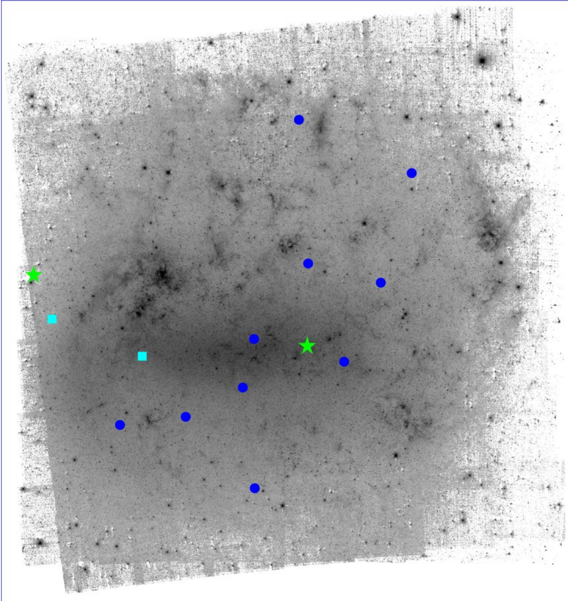
Figure 10. from Discovery and Analysis of 21 m Feature Sources in the Magellanic Clouds Volk et al. 2011 ApJ 735 127 doi:10.1088/0004-637X/735/2/127 https://dx.doi.org/10.1088/0004-637X/735/2/127 © 2011. The American Astronomical Society. All rights reserved.
