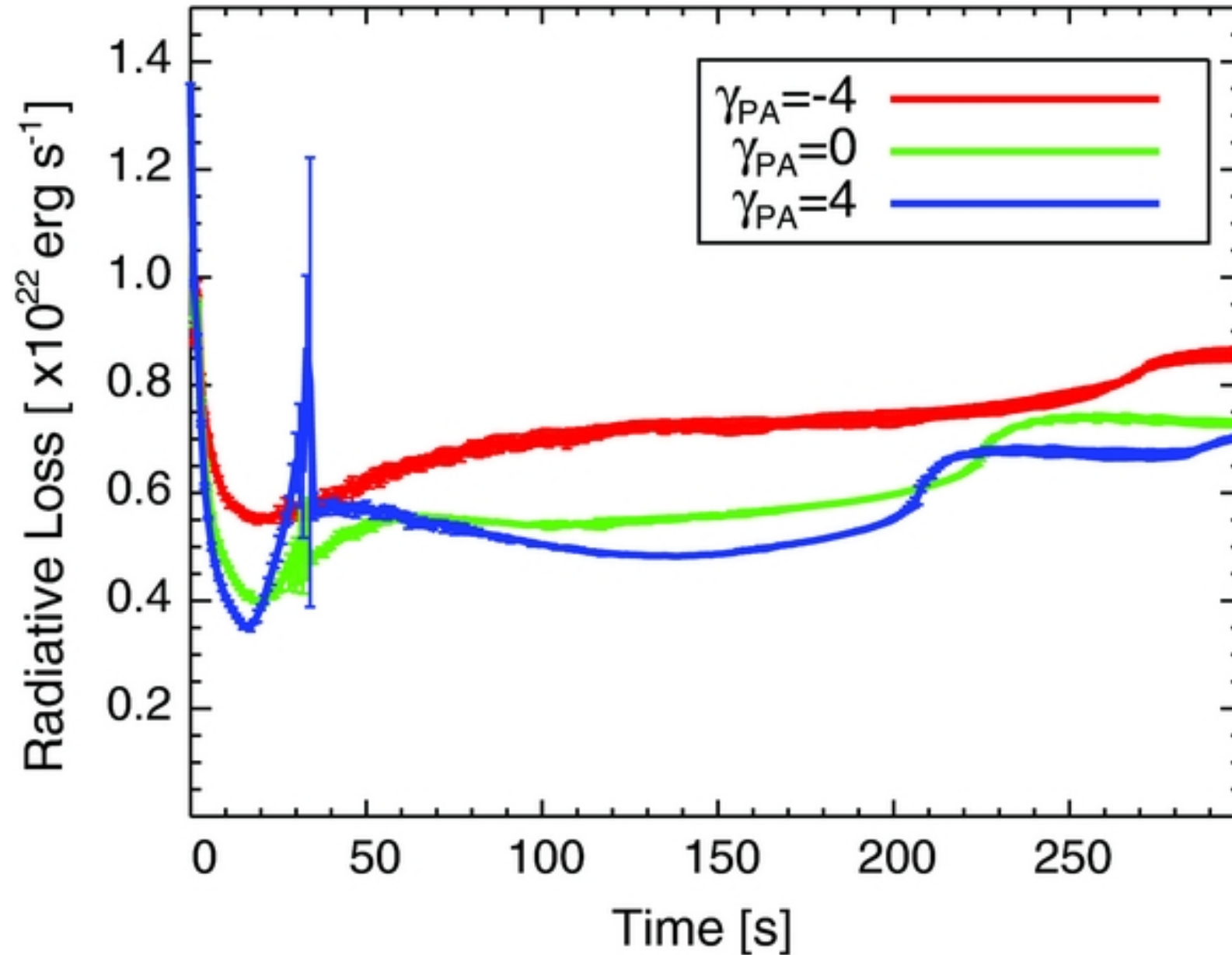
Figure 9. from Simulating the Effects of Initial Pitch-angle Distributions on Solar Flares Winter, Martens, & Reeves 2011 ApJ 735 103 doi:10.1088/0004-637X/735/2/103 https://dx.doi.org/10.1088/0004-637X/735/2/103 © 2011. The American Astronomical Society. All rights reserved.
