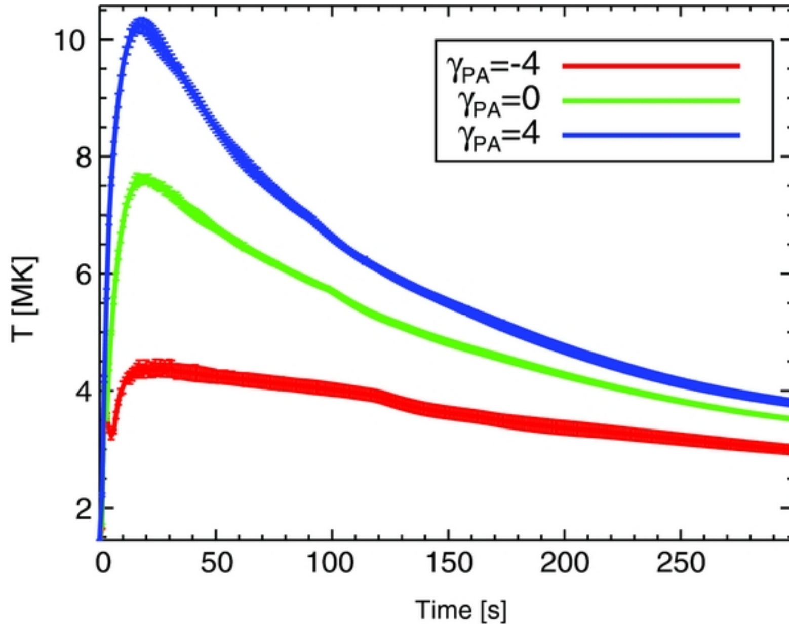
Figure 8. from Simulating the Effects of Initial Pitch-angle Distributions on Solar Flares Winter, Martens, & Reeves 2011 ApJ 735 103 doi:10.1088/0004-637X/735/2/103 https://dx.doi.org/10.1088/0004-637X/735/2/103 © 2011. The American Astronomical Society. All rights reserved.
