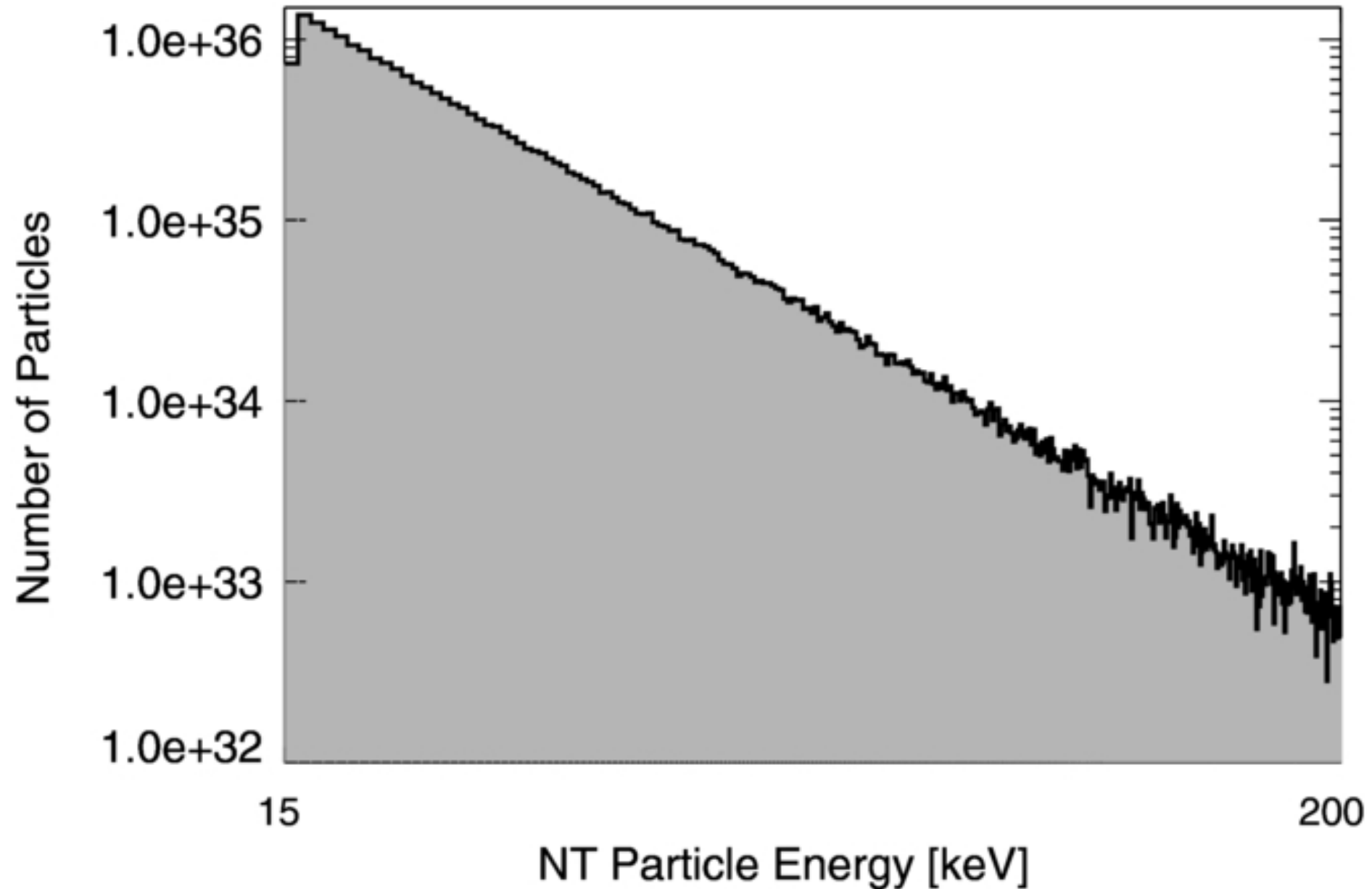
Figure 6. from Simulating the Effects of Initial Pitch-angle Distributions on Solar Flares Winter, Martens, & Reeves 2011 ApJ 735 103 doi:10.1088/0004-637X/735/2/103 https://dx.doi.org/10.1088/0004-637X/735/2/103 © 2011. The American Astronomical Society. All rights reserved.
