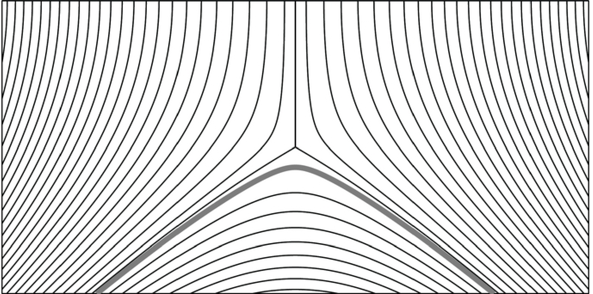
Figure 5. from Simulating the Effects of Initial Pitch-angle Distributions on Solar Flares Winter, Martens, & Reeves 2011 ApJ 735 103 doi:10.1088/0004-637X/735/2/103 https://dx.doi.org/10.1088/0004-637X/735/2/103 © 2011. The American Astronomical Society. All rights reserved.
