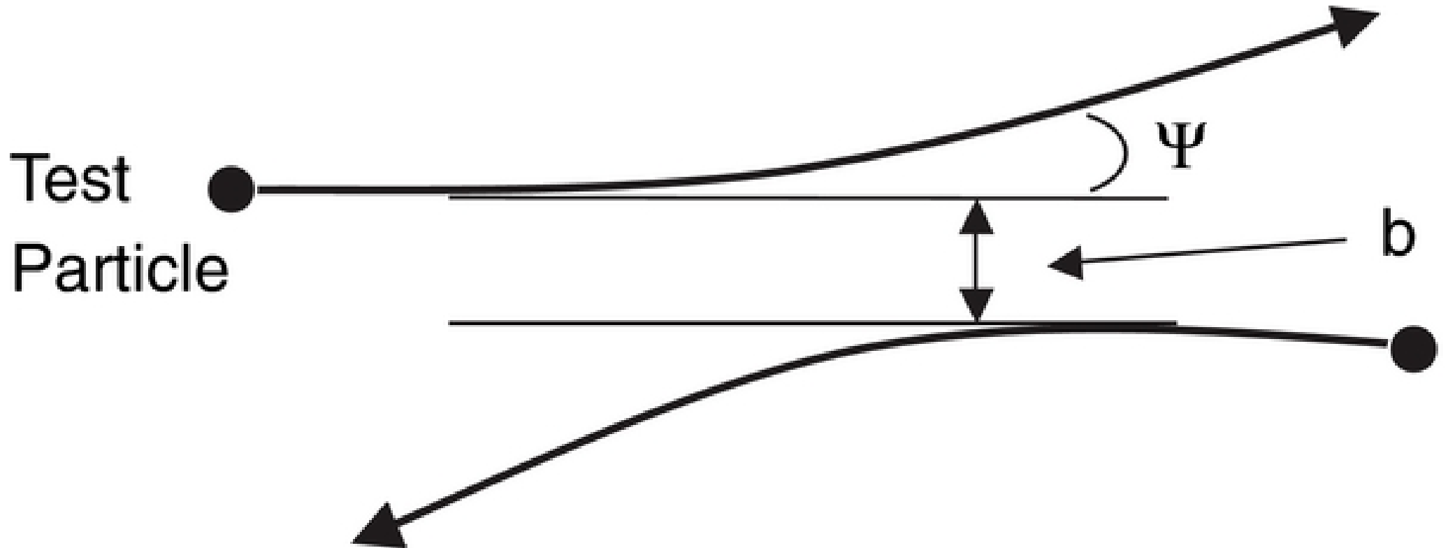
Figure 4. from Simulating the Effects of Initial Pitch-angle Distributions on Solar Flares Winter, Martens, & Reeves 2011 ApJ 735 103 doi:10.1088/0004-637X/735/2/103 https://dx.doi.org/10.1088/0004-637X/735/2/103 © 2011. The American Astronomical Society. All rights reserved.
