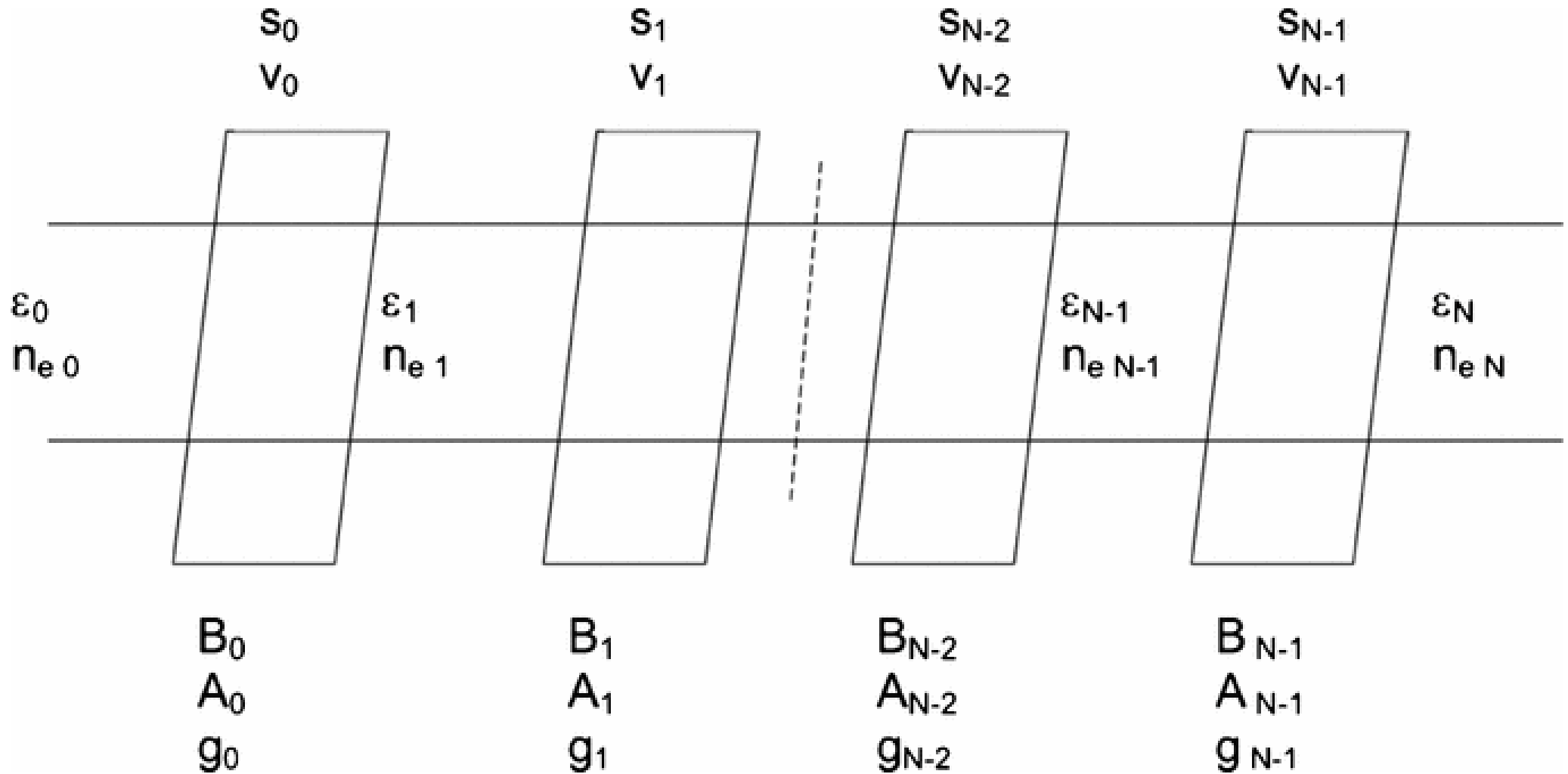
Figure 1. from Simulating the Effects of Initial Pitch-angle Distributions on Solar Flares Winter, Martens, & Reeves 2011 ApJ 735 103 doi:10.1088/0004-637X/735/2/103 https://dx.doi.org/10.1088/0004-637X/735/2/103 © 2011. The American Astronomical Society. All rights reserved.
