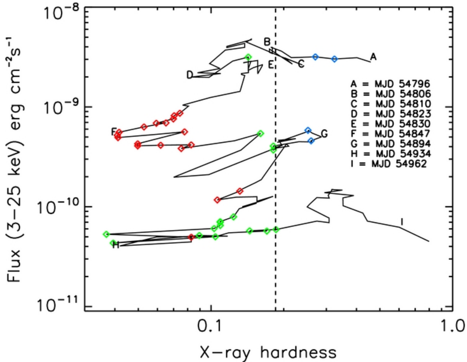
Figure 6. from Discovery and Evolution of the New Black Hole Candidate Swift J1539.2–6227 during its 2008 Outburst Krimm et al. 2011 ApJ 735 104 doi:10.1088/0004-637X/735/2/104 https://dx.doi.org/10.1088/0004-637X/735/2/104 © 2011. The American Astronomical Society. All rights reserved.
