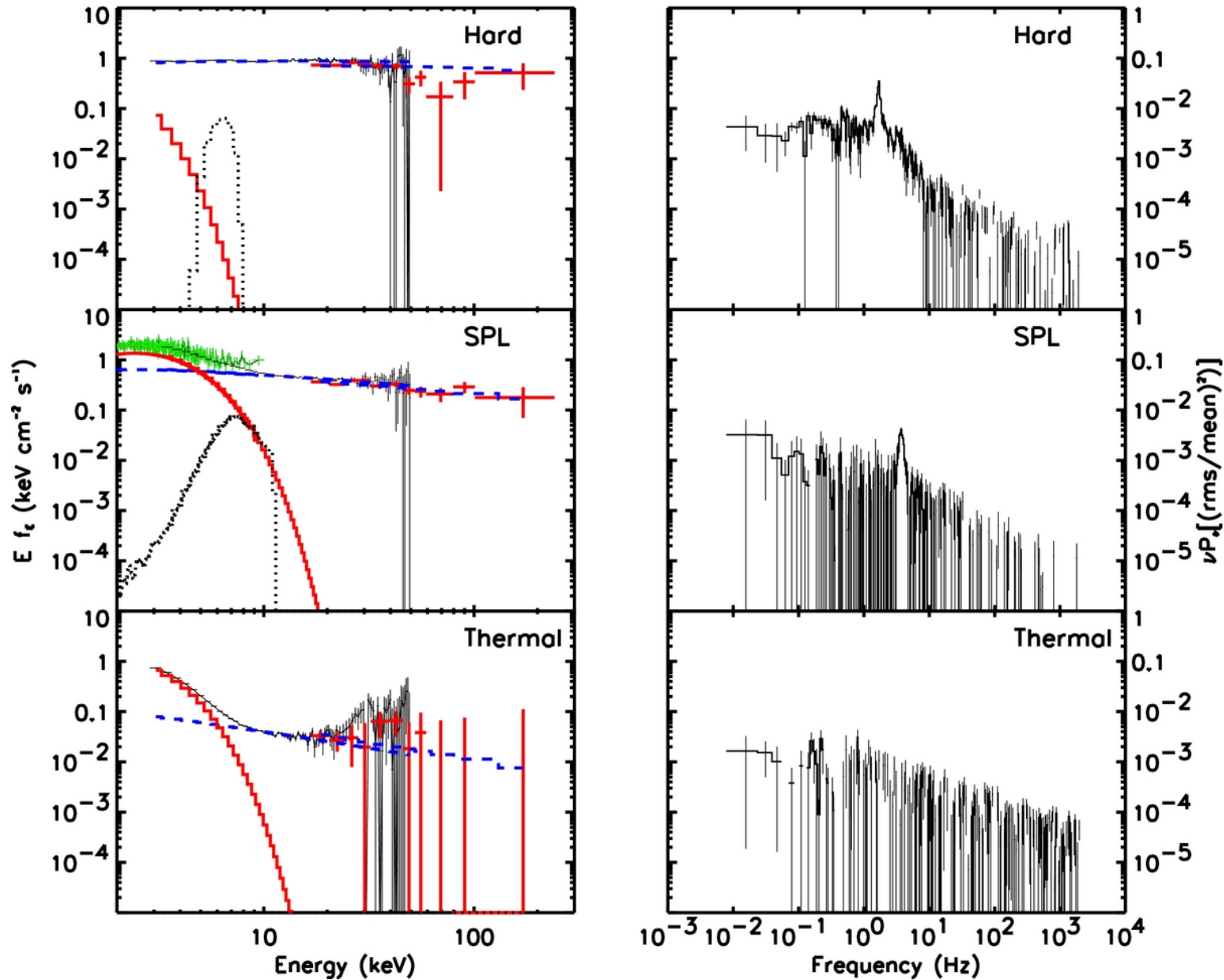
Figure 5. from Discovery and Evolution of the New Black Hole Candidate Swift J1539.2–6227 during its 2008 Outburst Krimm et al. 2011 ApJ 735 104 doi:10.1088/0004-637X/735/2/104 https://dx.doi.org/10.1088/0004-637X/735/2/104
