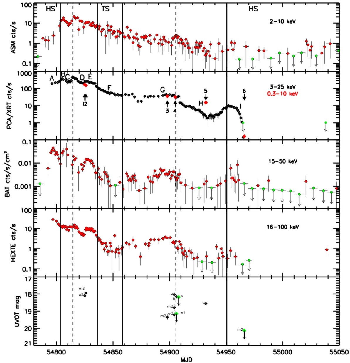
Figure 1. from Discovery and Evolution of the New Black Hole Candidate Swift J1539.2–6227 during its 2008 Outburst Krimm et al. 2011 ApJ 735 104 doi:10.1088/0004-637X/735/2/104 https://dx.doi.org/10.1088/0004-637X/735/2/104
