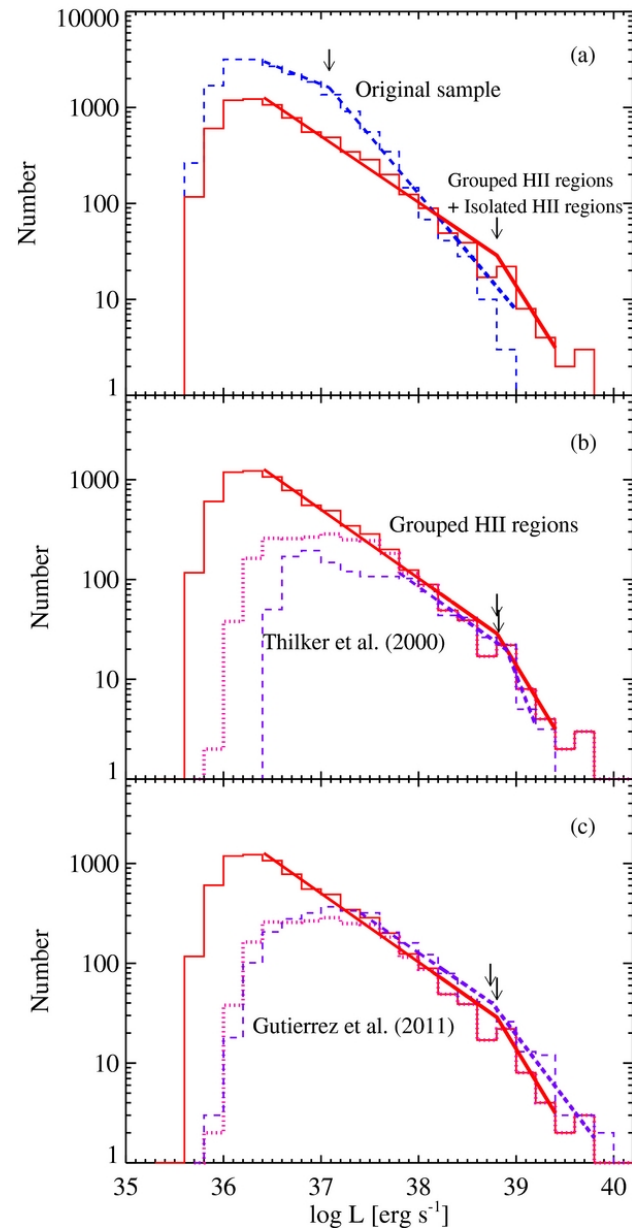
Figure 5. from H II Region Luminosity Function of the Interacting Galaxy M51 Lee, Hwang, & Lee 2011 ApJ 735 75 doi:10.1088/0004-637X/735/2/75 https://dx.doi.org/10.1088/0004-637X/735/2/75 © 2011. The American Astronomical Society. All rights reserved.
