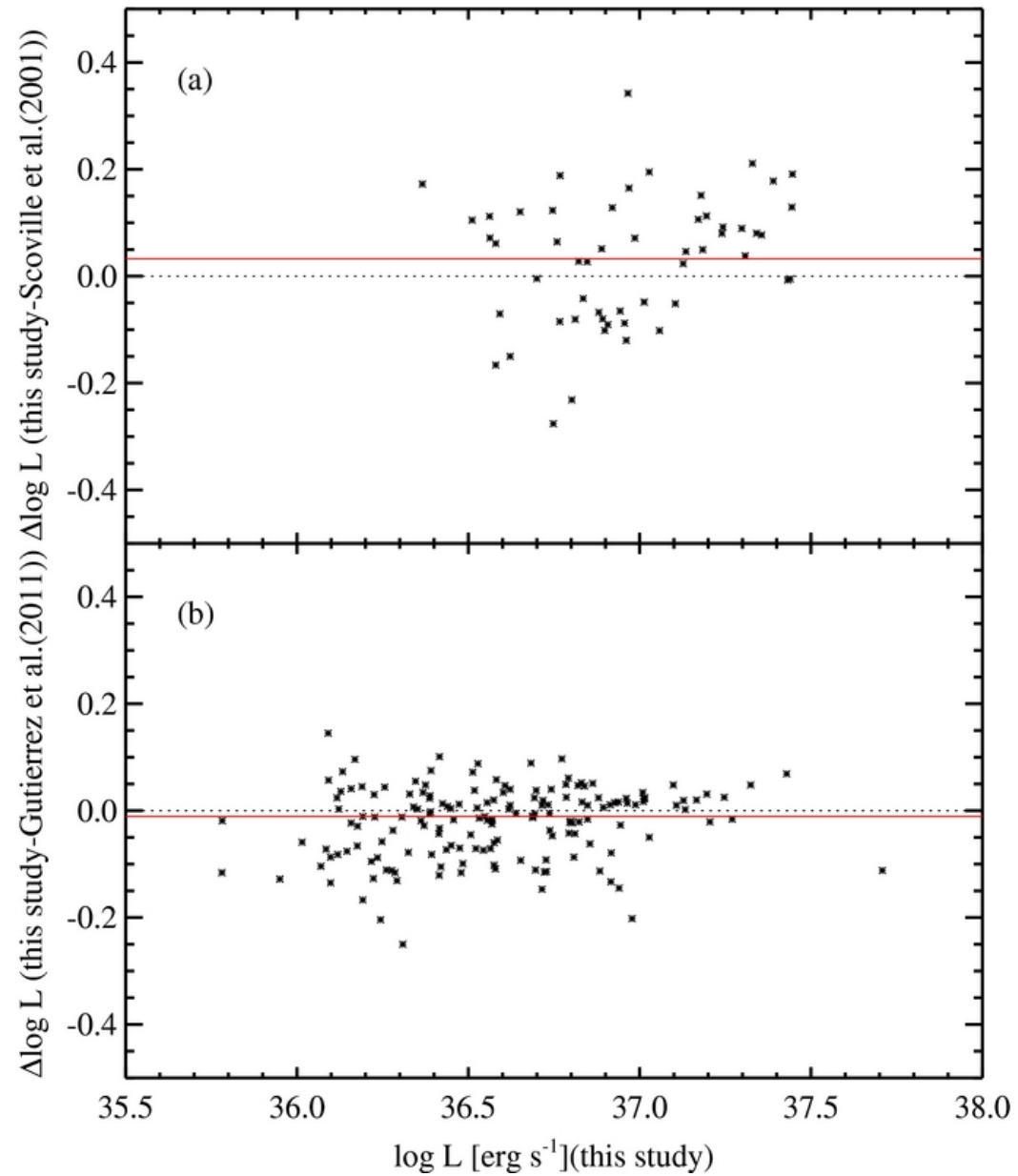
Figure 2. from H II Region Luminosity Function of the Interacting Galaxy M51 Lee, Hwang, & Lee 2011 ApJ 735 75 doi:10.1088/0004-637X/735/2/75 https://dx.doi.org/10.1088/0004-637X/735/2/75 © 2011. The American Astronomical Society. All rights reserved.
