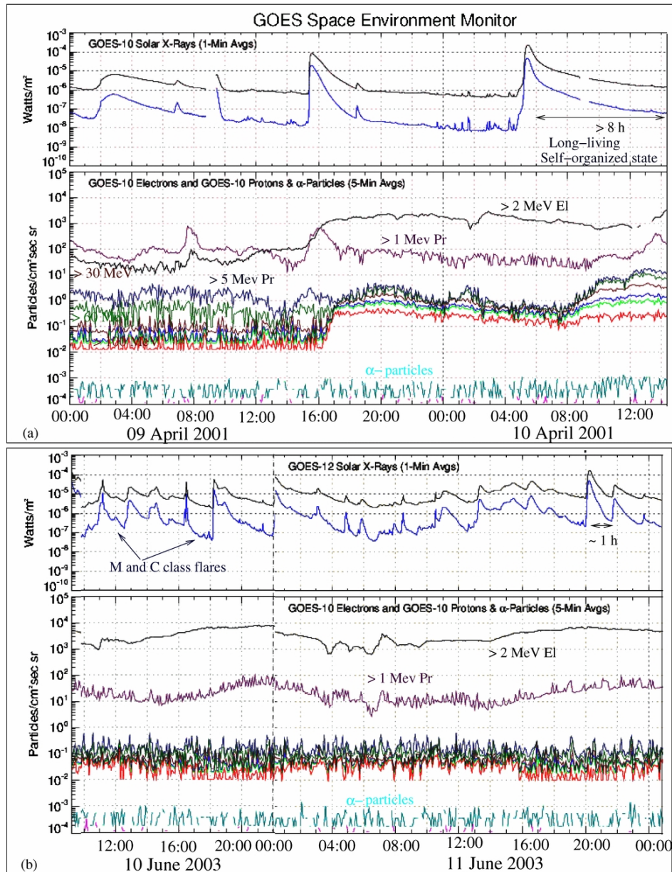
Figure 6. from Flares Producing Well-organized Post-flare Arcades (Slinkies) Have Early Precursors Ryutova et al. 2011 ApJ 733 125 doi:10.1088/0004-637X/733/2/125 https://dx.doi.org/10.1088/0004-637X/733/2/125 © 2011. The American Astronomical Society. All rights reserved.
