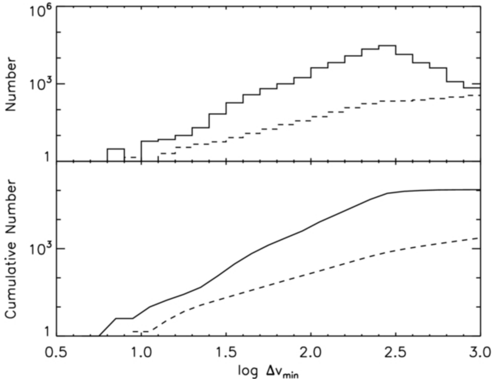
Figure 9. from Identifying Collisional Families in the Kuiper Belt Marcus et al. 2011 ApJ 733 40 doi:10.1088/0004-637X/733/1/40 https://dx.doi.org/10.1088/0004-637X/733/1/40 © 2011. The American Astronomical Society. All rights reserved.
