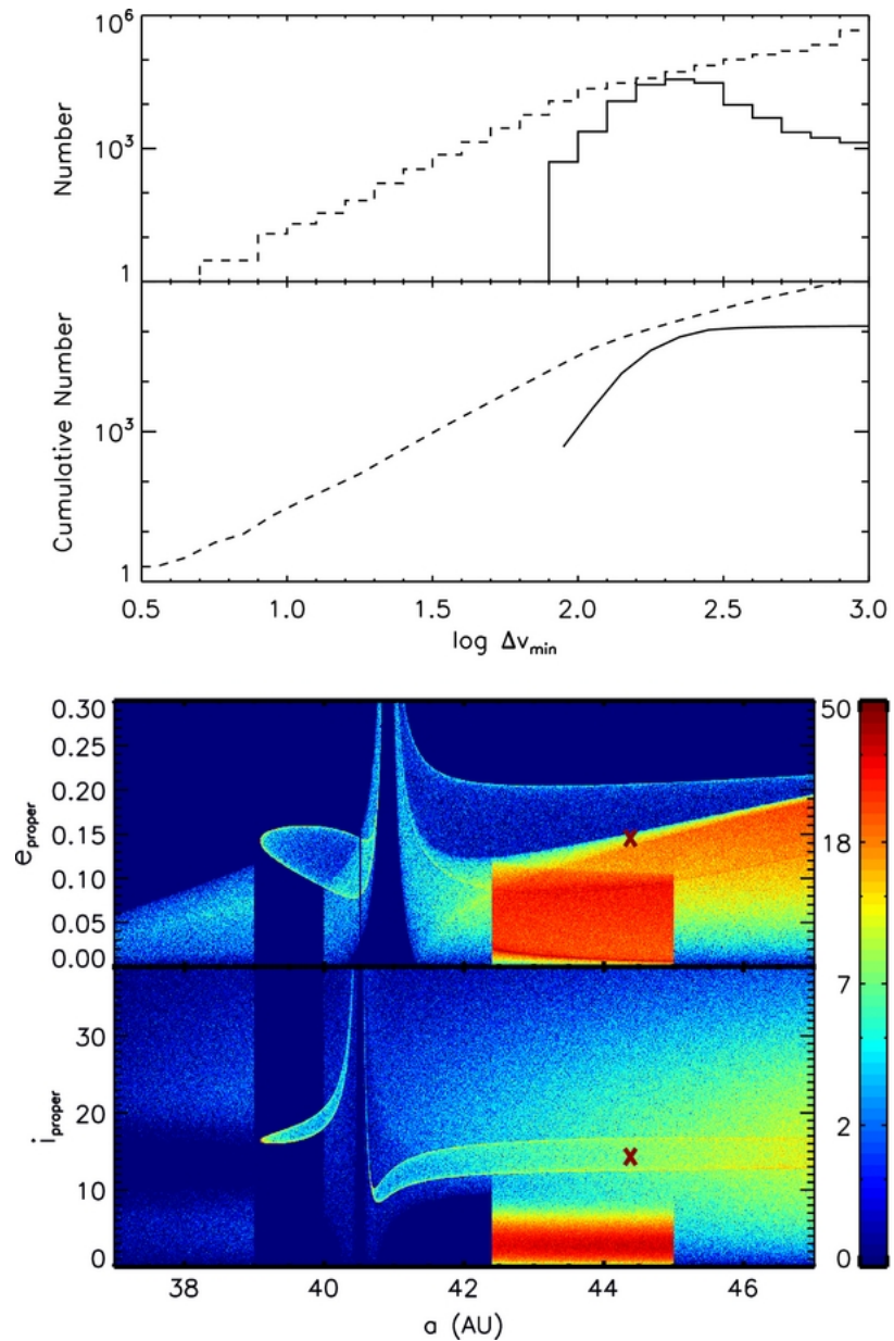
Figure 5. from Identifying Collisional Families in the Kuiper Belt Marcus et al. 2011 ApJ 733 40 doi:10.1088/0004-637X/733/1/40 https://dx.doi.org/10.1088/0004-637X/733/1/40 © 2011. The American Astronomical Society. All rights reserved.
