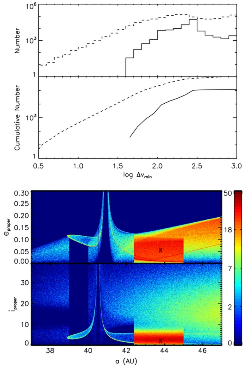
Figure 4. from Identifying Collisional Families in the Kuiper Belt Marcus et al. 2011 ApJ 733 40 doi:10.1088/0004-637X/733/1/40 https://dx.doi.org/10.1088/0004-637X/733/1/40 © 2011. The American Astronomical Society. All rights reserved.
