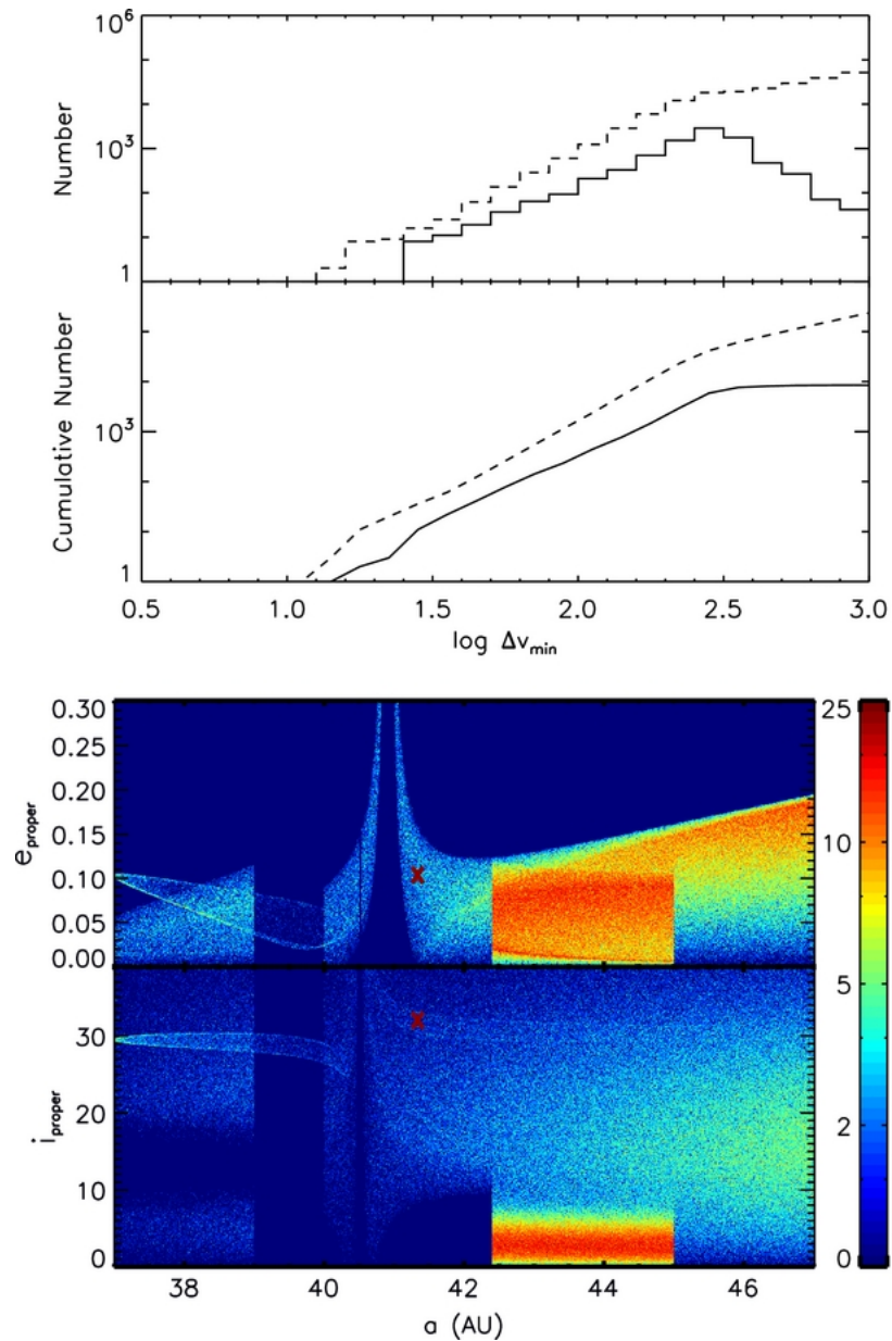
Figure 3. from Identifying Collisional Families in the Kuiper Belt Marcus et al. 2011 ApJ 733 40 doi:10.1088/0004-637X/733/1/40 https://dx.doi.org/10.1088/0004-637X/733/1/40 © 2011. The American Astronomical Society. All rights reserved.
