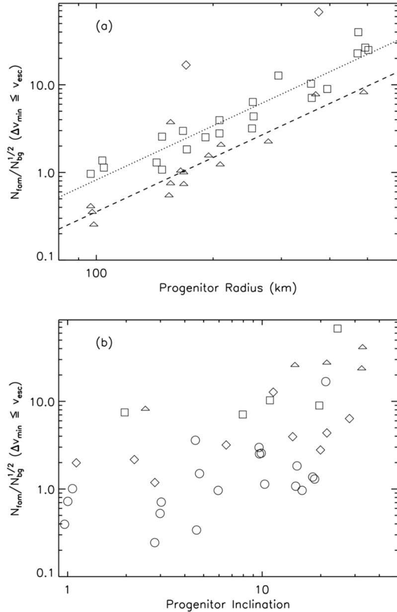
Figure 11. from Identifying Collisional Families in the Kuiper Belt Marcus et al. 2011 ApJ 733 40 doi:10.1088/0004-637X/733/1/40 https://dx.doi.org/10.1088/0004-637X/733/1/40 © 2011. The American Astronomical Society. All rights reserved.
