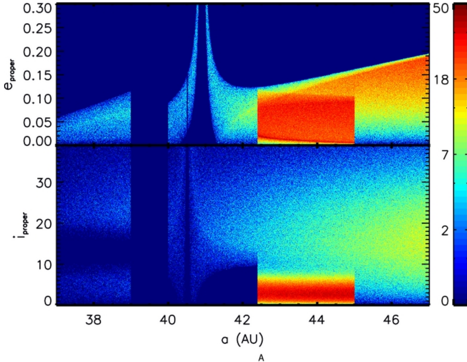
Figure 1. from Identifying Collisional Families in the Kuiper Belt Marcus et al. 2011 ApJ 733 40 doi:10.1088/0004-637X/733/1/40 https://dx.doi.org/10.1088/0004-637X/733/1/40 © 2011. The American Astronomical Society. All rights reserved.
