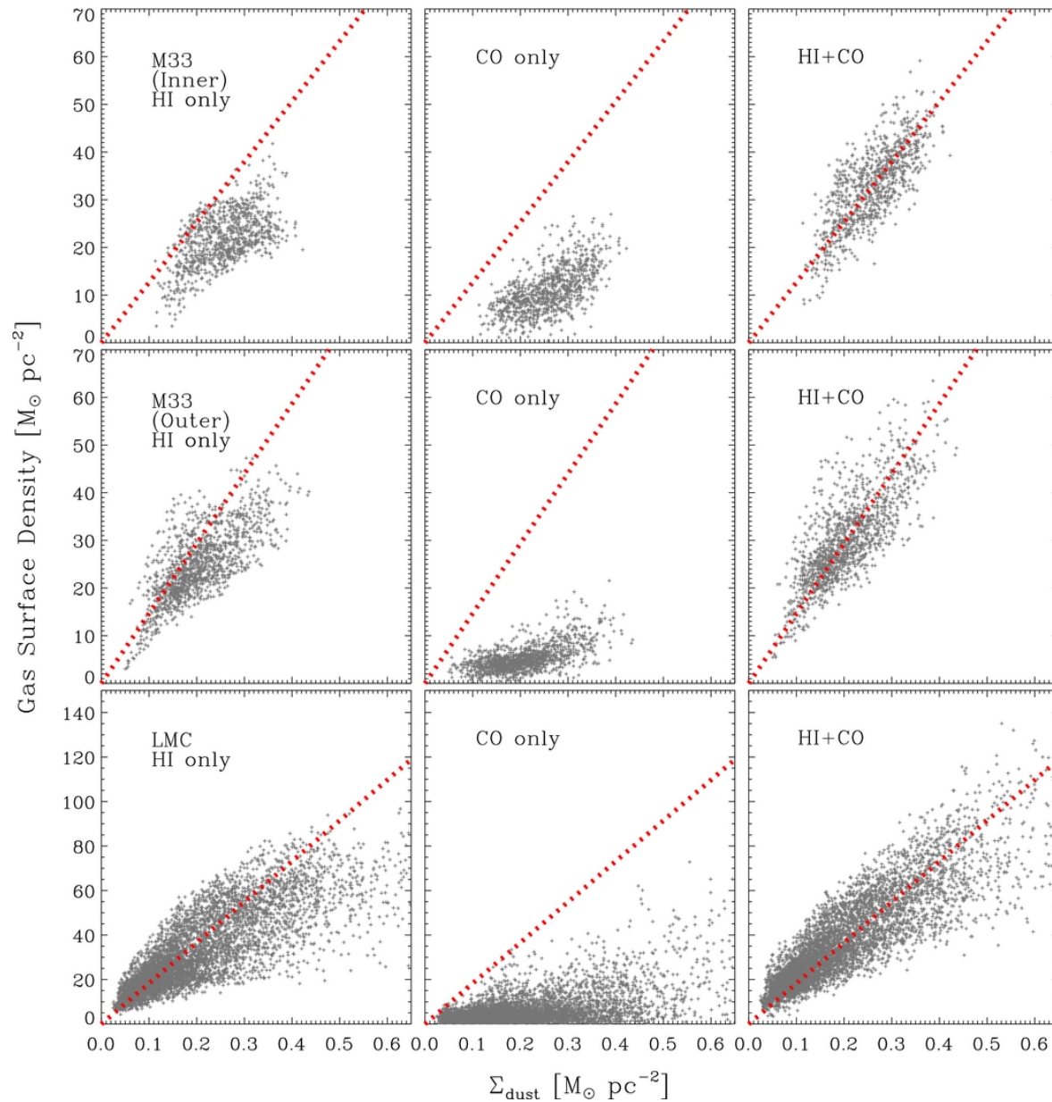
Figure 4. from The CO-to-H 2 Conversion Factor from Infrared Dust Emission across the Local Group Leroy et al. 2011 ApJ 737 12 doi:10.1088/0004-637X/737/1/12 https://dx.doi.org/10.1088/0004-637X/737/1/12 © 2011. The American Astronomical Society. All rights reserved.
