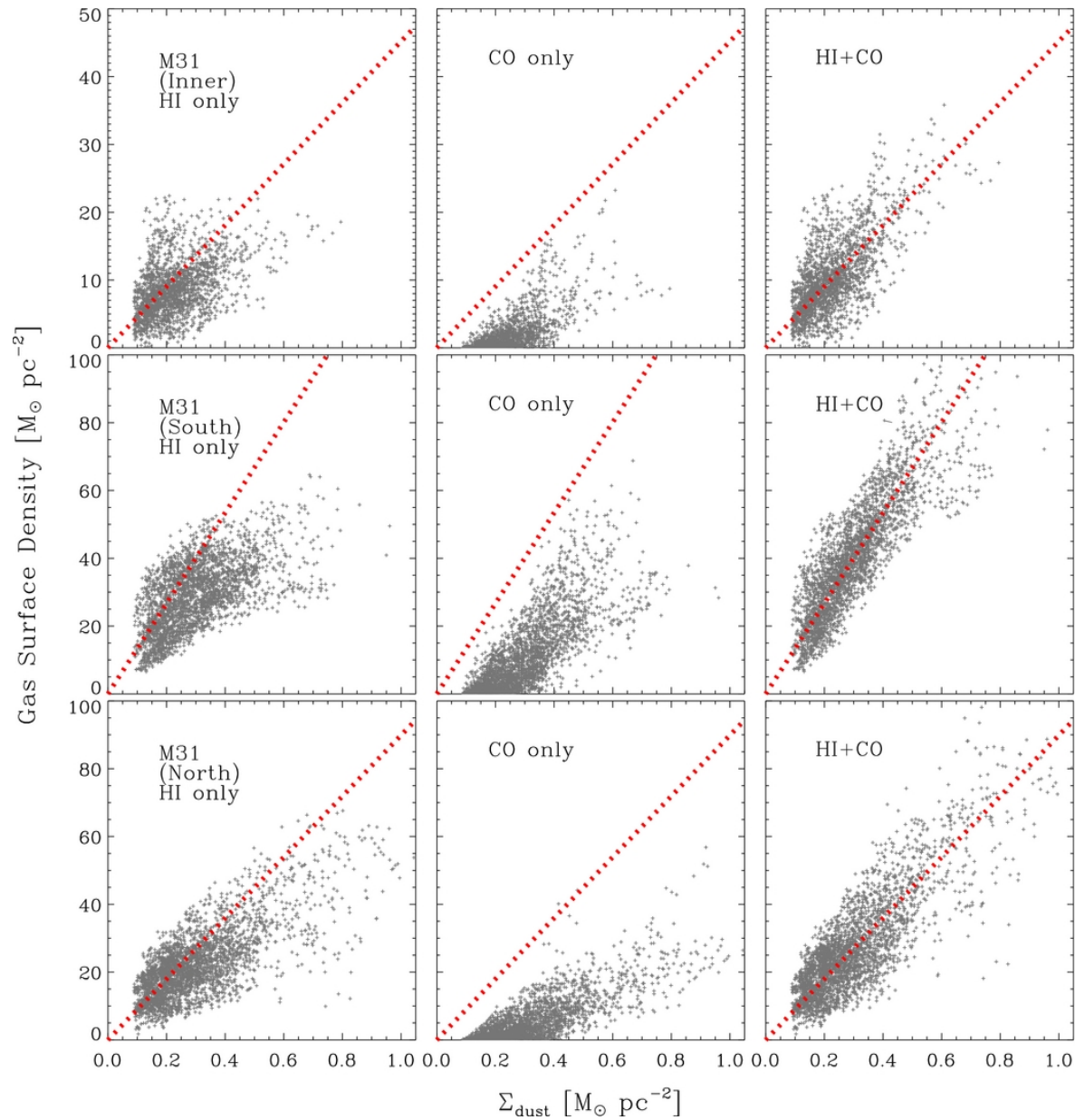
Figure 3. from The CO-to-H 2 Conversion Factor from Infrared Dust Emission across the Local Group Leroy et al. 2011 ApJ 737 12 doi:10.1088/0004-637X/737/1/12 https://dx.doi.org/10.1088/0004-637X/737/1/12 © 2011. The American Astronomical Society. All rights reserved.
