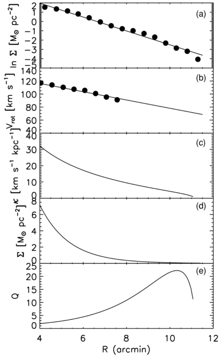
Figure 9. from The Structure and Metallicity Gradient in the Extreme Outer Disk of NGC 7793 Vlaji, Bland-Hawthorn, & Freeman 2011 ApJ 732 7 doi:10.1088/0004-637X/732/1/7 https://dx.doi.org/10.1088/0004-637X/732/1/7
