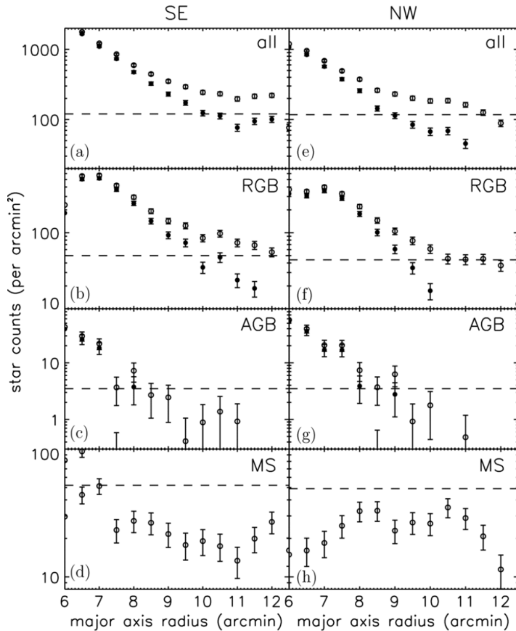
Figure 5. from The Structure and Metallicity Gradient in the Extreme Outer Disk of NGC 7793 Vlaji, Bland-Hawthorn, & Freeman 2011 ApJ 732 7 doi:10.1088/0004-637X/732/1/7 https://dx.doi.org/10.1088/0004-637X/732/1/7
